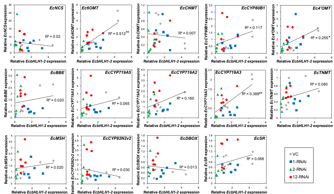
Supplementary Figure S12. Correlation analysis between the expression of EcbHLH1-1 (A) or EcbHLH1-2 (B) and that of all sanguinarine biosynthetic enzyme genes. The relative expression level shows the values standardized by that of the VC4-1 sample as 1. Asterisks indicate significant correlation between the expression of two genes (df=22, *P < 0.05 , **P < 0.01 )
