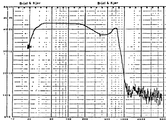
Figure 2. The frequency response of the hot-wire flow meter. Note that the response curve is quasi-flat up to 750 Hz.
