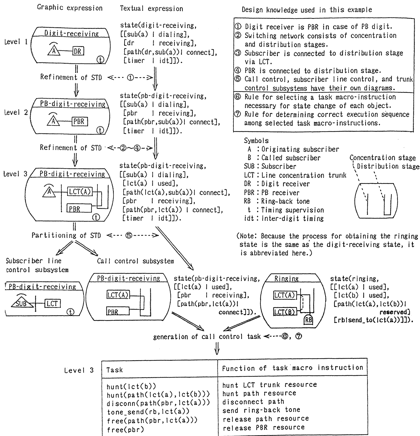
Fig.4 Example of state transition diagram(STD) design and task generation
