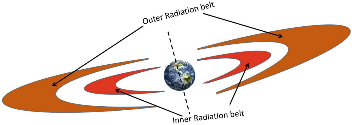
Figure 1: Schematic diagram of the two-belt structure of the Earth's radiation belts.
