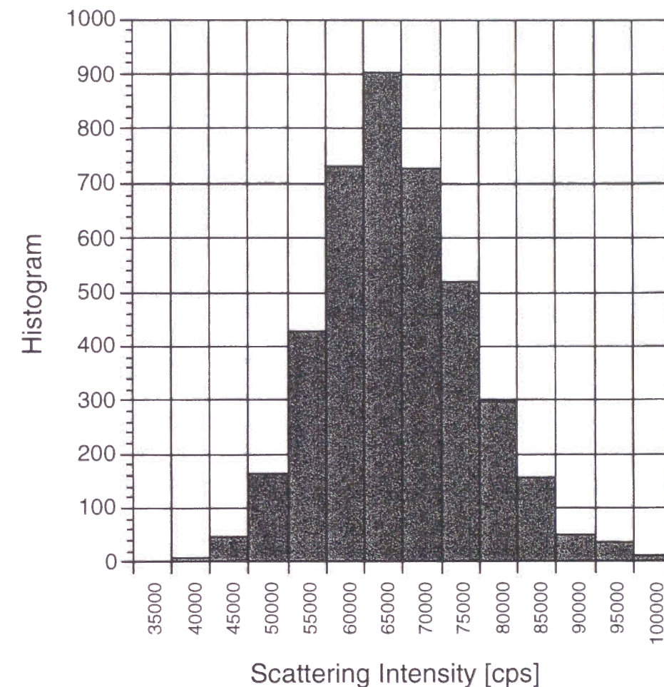
Figure 4-5 Examples of histogram obtained from EVLSM. Particle : polystyrene latex (diameter = 1000 nm) Surface : chemically-modified Pyrex glass ( \zeta = -8 mV) Added NaCl concentration : 0mM
