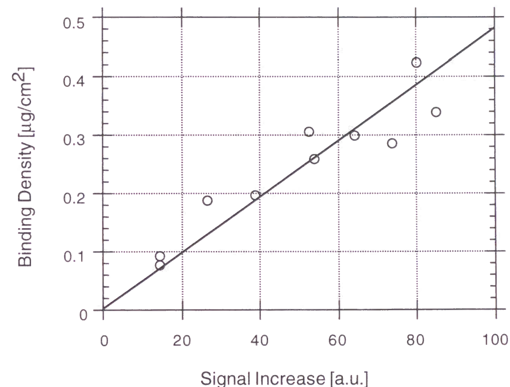
Figure 6-4 Calibration curve used for conversion of the signal intensity into the density of antibody bound to a hapten-doped lipid monolayer (DNP-cap-DPPE : DSPC = 10 : 90 [mol%]).
