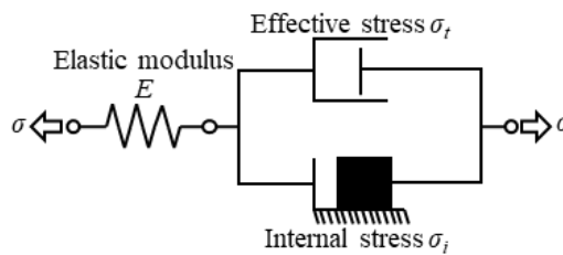
Figure 4. Elasto-viscoplasticity model
