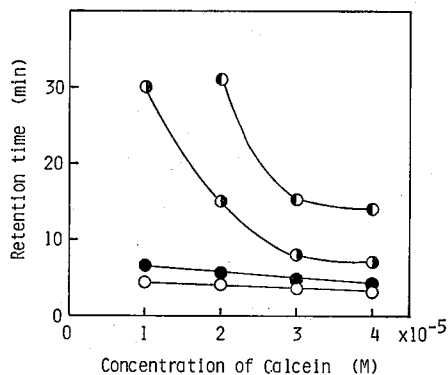
Fig. 6. Effect of Calcein concentration on retention time KOH; 0.1 M, flow rate; 0.42 ml/min, column; 33cm \times 2mm, temp.; 25°C, dead time; 2.5 min.
