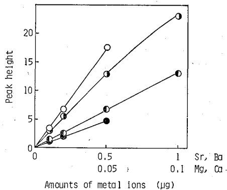
Fig. 10. Calibration curves. Calcein; 4 \times 10^{-5} M, KOH; 0.1M, column; 33cm, flow rate; 0.42 ml/min, temp.; 25^\circ\text{C} , \circ ; Mg \bullet ; Ca, \circ ; Sr, \bullet ; Ba.
