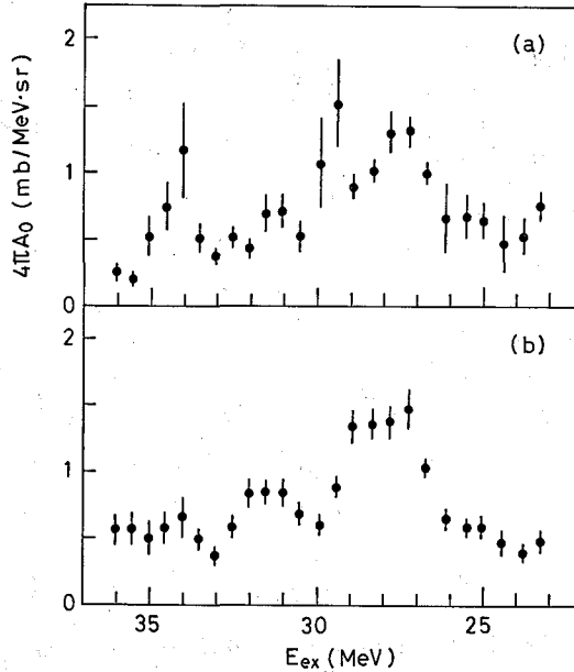
Fig. 3. Coefficients A_0 of the Legendre polynomials, multiplied by a factor 4\pi . The upper part (a) corresponds to the fit with k_{max}=4 and lower part (b) to the fit with k_{max}=2 .
