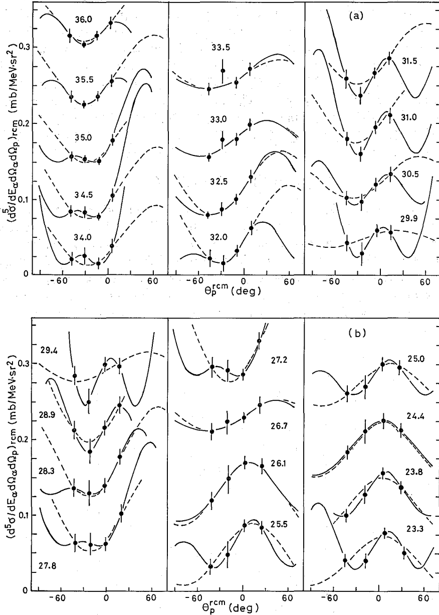
Fig. 2. Angular correlations for the {}^4\text{He}(\alpha, \alpha'){}^4\text{He}^*(p){}^3\text{H} reaction at \theta_\alpha = 25^\circ . Full circles represent experimental points and full lines the Legendre polynomials fit with k_{\max}=4 and dashed lines the one with k_{\max}=2 . The angular correlations are designated with the corresponding excitation energies for {}^4\text{He}^* and are shown by shifted upward successively by a factor 0.075.
