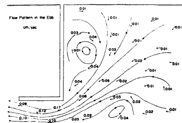
Fig. 8. Flow pattern in the ebb of Run 8.
