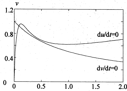
Fig.2 Null-clines for the model Eq.(1) with Eqs.(2) and (3). Cell density n is fixed to 1.0. Refer to Table 1 for parameter values.
