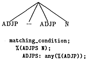
Figure 3.3: Expression of Tree Structure with ‘any’
