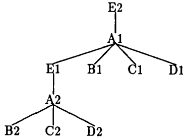
Figure 3.12: Final Result of Application of the Rewriting Rule
