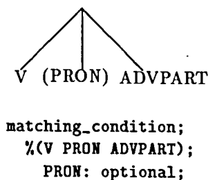
Figure 3.4: Expression of Tree Structure with ‘optional’
