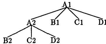
Figure 3.10: Input Tree Structure for the Rewriting Rule
