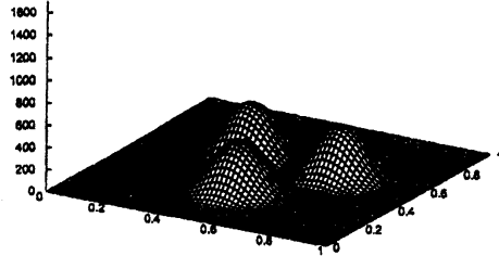
(i) t_0 = 0.000000 (\|u_{0h}\|_1 = 50.000)
