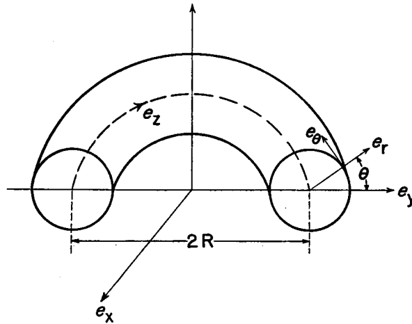
Fig. 1. Toroidal Coordinates.
