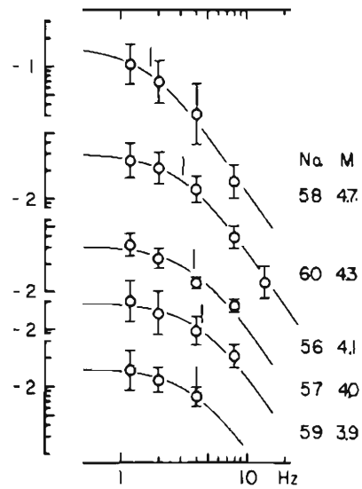
Fig. 14. continued. (c) Gifu and Aichi prefectures, (f) in and off Kii peninsula and Kii channel, (g) others including the events near the Ontake-volcano.
