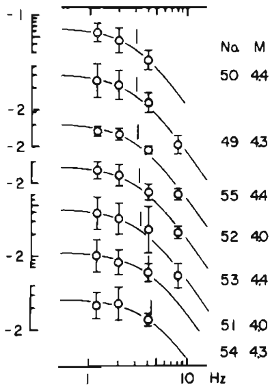
Fig. 14. continued. (c) Gifu and Aichi prefectures, (f) in and off Kii peninsula and Kii channel, (g) others including the events near the Ontake-volcano.
