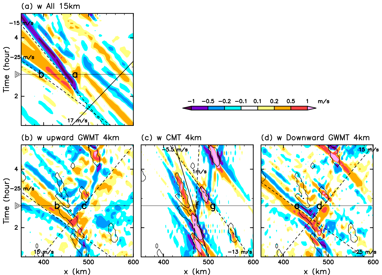
FIG. 11. As in Fig. 7, but for 350 \leq x \leq 600 km, 1:00 \leq t \leq 5:00 on day 304.
