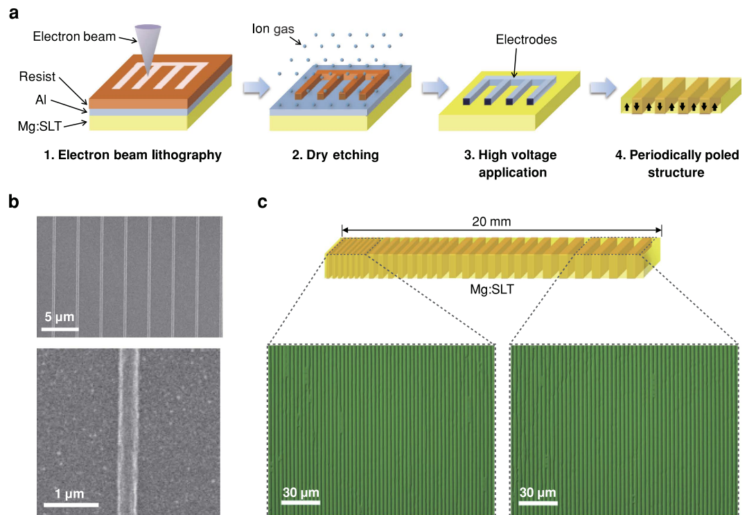
Figure 2. Fabrication of chirped QPM lithium tantalate device using nano-electrode-poling technique.
