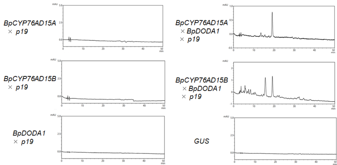
Fig. 5 Transient over-expression analysis by agroinfiltration in leaves. a Photos of infiltrated leaves. b RT-PCR validation of transgenic over-expression in infiltrated leaves. c Color of leaf extracts. d HPLC chromatograms of over-expression leaves analyzed at 470 nm
