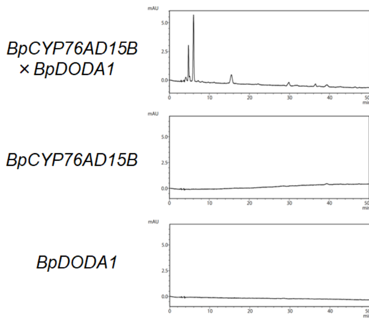
Fig. 6 Over-expression analysis in transgenic N. tabacum plants. a RT-PCR validation of transgene expression in flowers. b Flower color of transgenic over-expression flowers. c Color of flower extract from over-expression transgenic plants. d HPLC chromatograms of over-expression flowers analyzed at 470 nm
