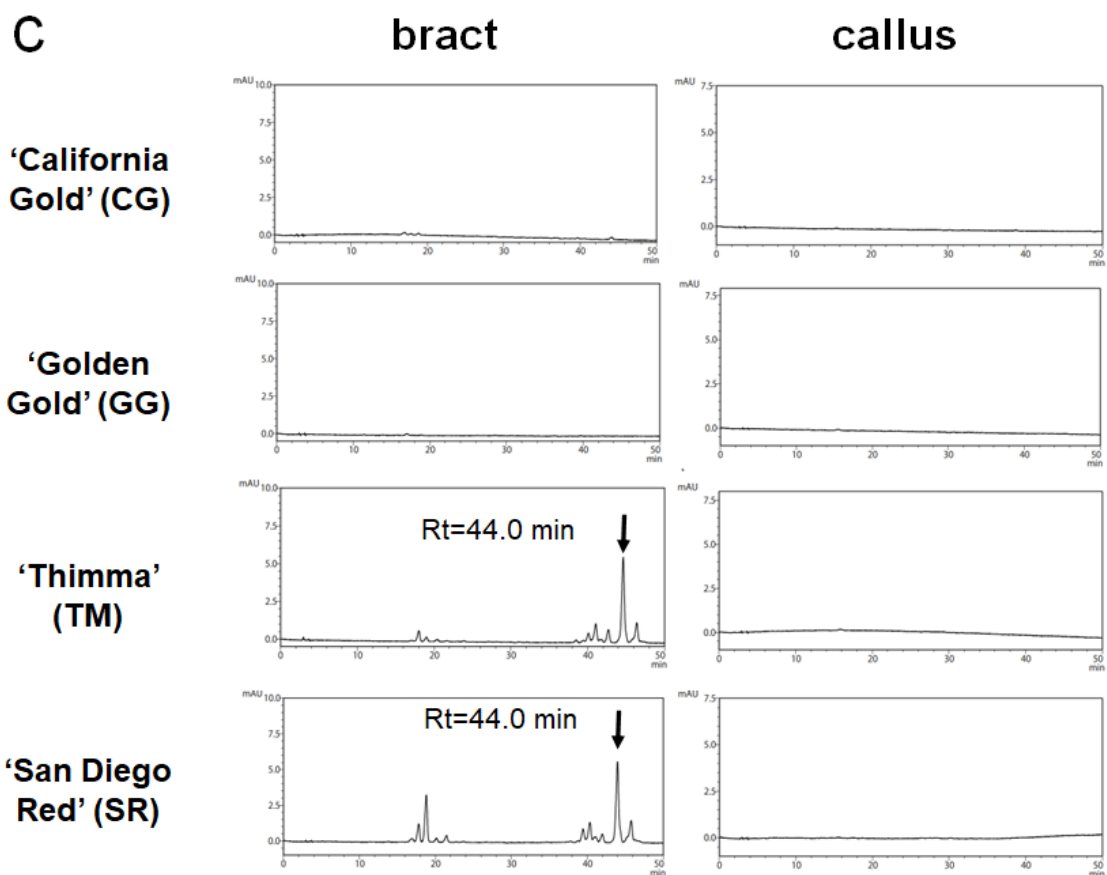
Fig. 2 Pigment analysis in bracts and callus. a Cultivars used in this study. b HPLC analysis on 470 nm for betaxanthin in bracts and callus. c HPLC analysis on 535 nm for betacyanin in bracts and callus
