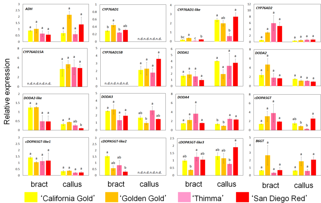
Fig. 4 Relative expression of betalain biosynthetic genes in 1-2 cm bracts and in callus among four cultivars. BpActin was used as an internal control. Bars represent standard errors ( n = 3 ). n.d. indicates not detected. Different letters above the bars indicate significant differences by Tukey's HSD test ( P < 0.05 )
