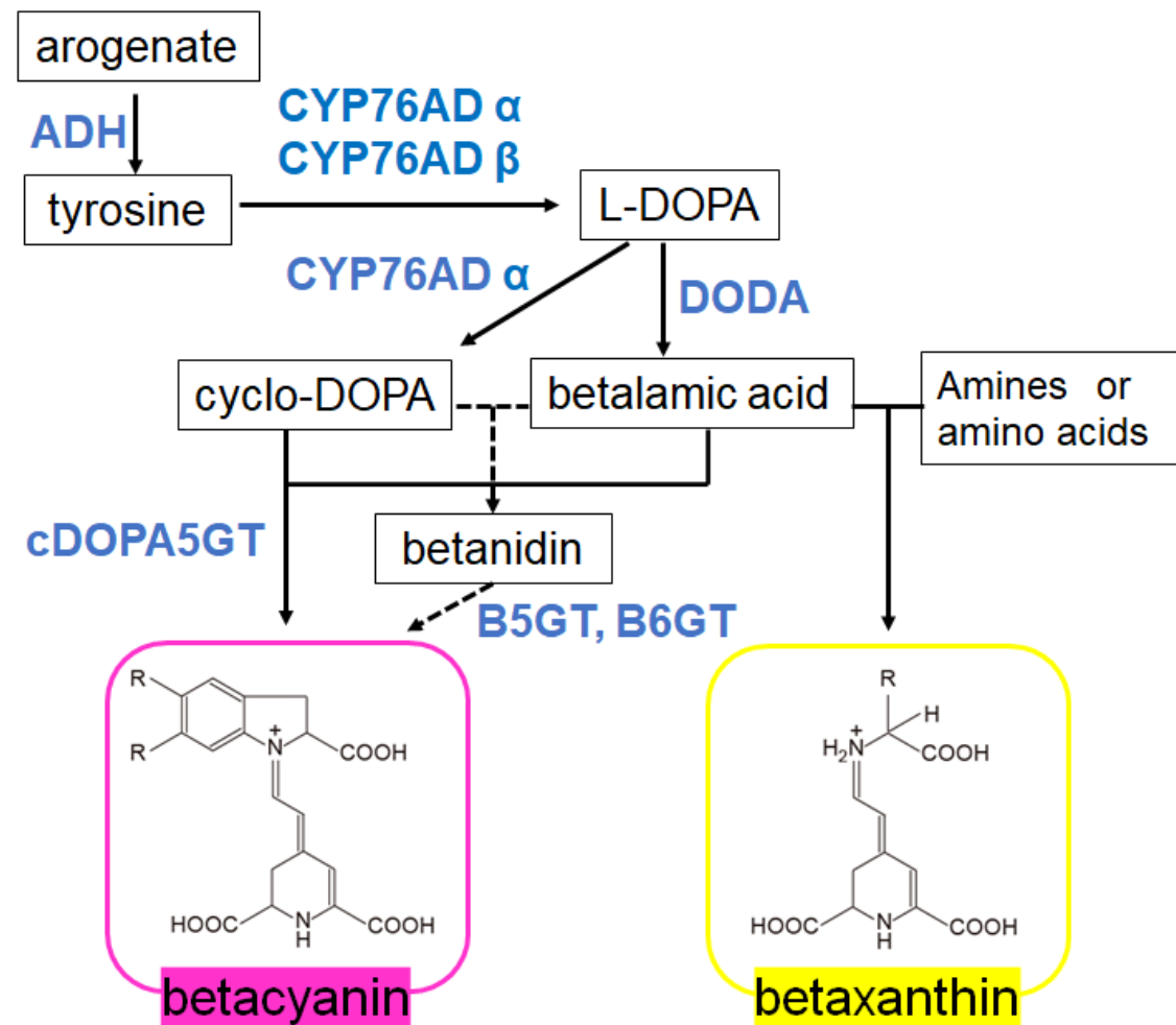
Fig.1 Betalain biosynthetic pathway. ADH: aroenate dehydrogenase, CYP76AD: cytochrome p450 76AD, DODA: L-DOPA 4,5-dioxygenase, cDOPA5GT: cyclo-DOPA 5-O-glucosyltransferase, B5GT: betanidin-5-O-glucosyltransferase, B6GT: betanidin-6-O-glucosyltransferase
