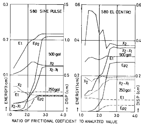
Fig. 22 Transmitted energy and displacement versus frictional coefficient ratio.
