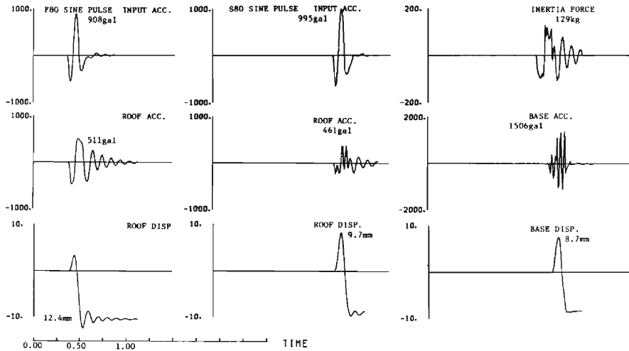
Fig. 12 Experimental time history due to sine pulse.
