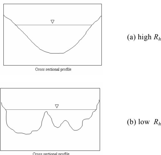
Fig.7 Management of hydraulic radius for increasing retention efficiency. If a maximum depth is constant, the low R_h with complex wetted perimeter is efficient for retention for lentic plankton
