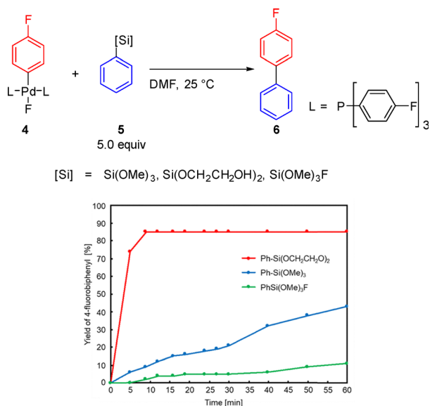
Scheme 2 Stoichiometric reactions of an arylpalladium fluoride with organosilanes.
