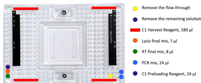
Figure 5. Pipetting map for cell lysis, reverse transcription, and PCR steps
