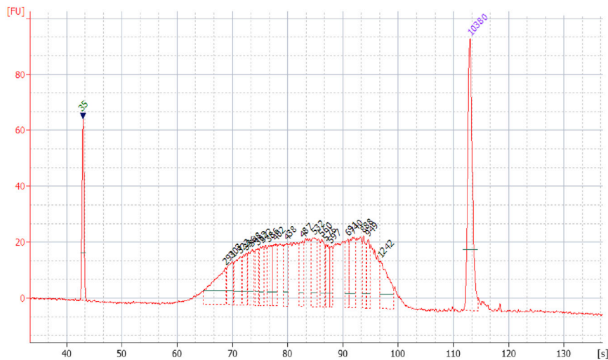
Figure 8. Quantitative of the single-cell cDNA library using Bioanalyzer
