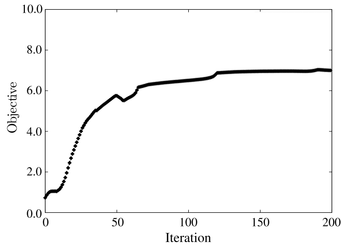
Fig. 2.10 Convergence history for objective functional I when setting \theta = 100 in the heat exchange maximization problem.
