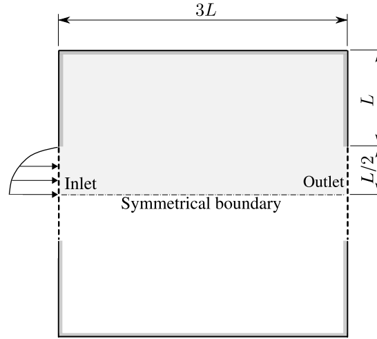
Fig. 2.6 Design model and fixed design domain D in the heat exchange maximization problem.
