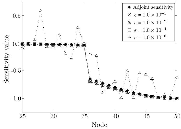
Fig. 3.4 Comparison of the finite differences with respect to the adjoint sensitivities in flow resistance minimization problem. The node in the horizontal axis corresponds to each evaluation node in the analysis domain as shown in Fig. 3.2.
