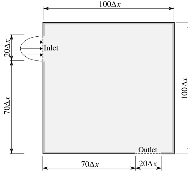
Fig. 3.12 Design settings in the pipe bend problem using the LBM.
