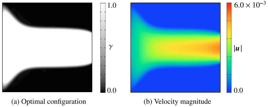
Fig. 3.7 Optimal configuration (black: fluid, white: solid) and the velocity magnitude in the diffuser problem using the LBM.
