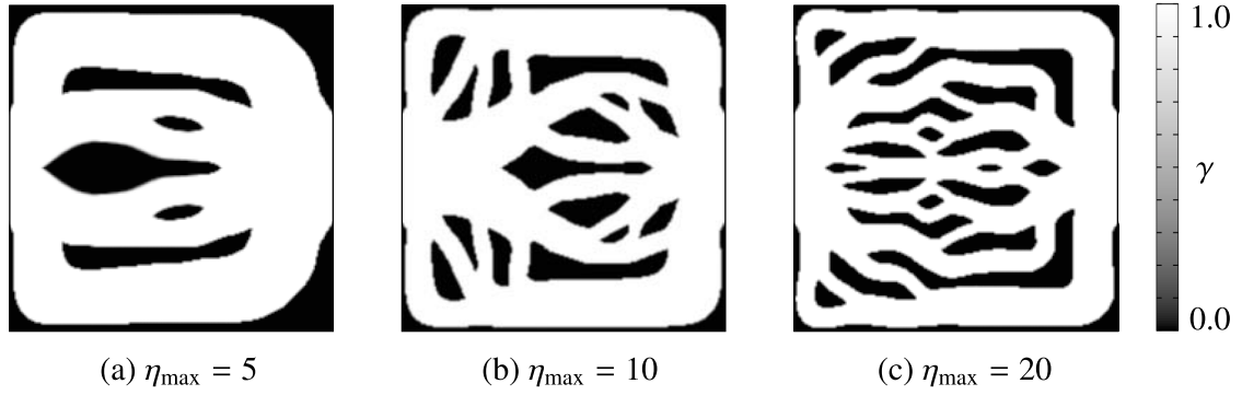
Fig. 4.8 Effect of parameter \eta_{\max} settings on optimal configurations: (a) \eta_{\max} = 5 , (b) \eta_{\max} = 10 , (c) \eta_{\max} = 20 .
