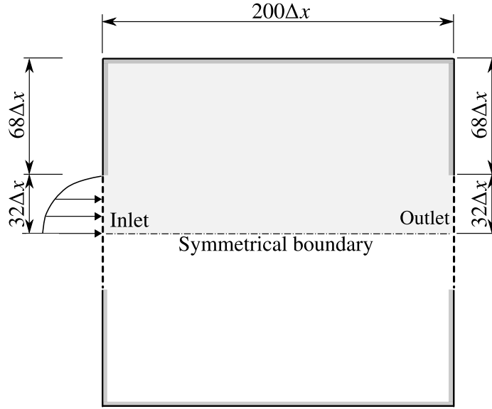
Fig. 4.4 Design settings in heat exchange maximization problem using the LBM. The analysis domain, where the symmetrical boundary condition is imposed, is discretized using 200\Delta x \times 100\Delta x .
