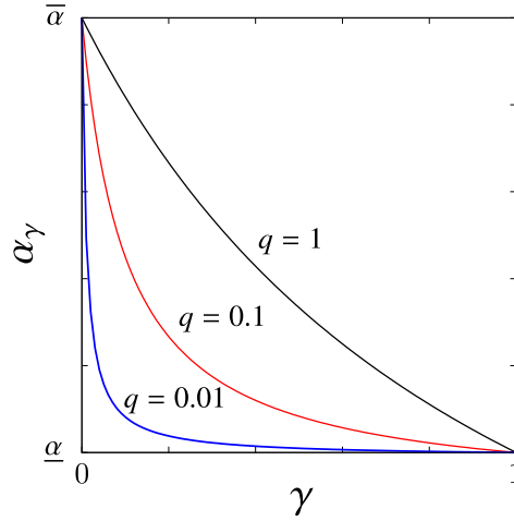
Fig. 2.5 The interpolation function \alpha(\gamma) plotted for q = 0.01, 0.1 , and 1 .
