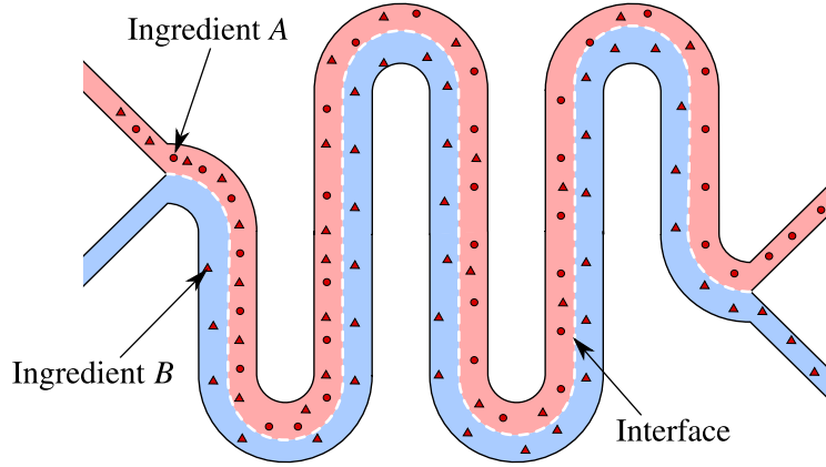
Fig. 5.1 Schematic diagram of liquid-liquid extraction in microchannel device.
