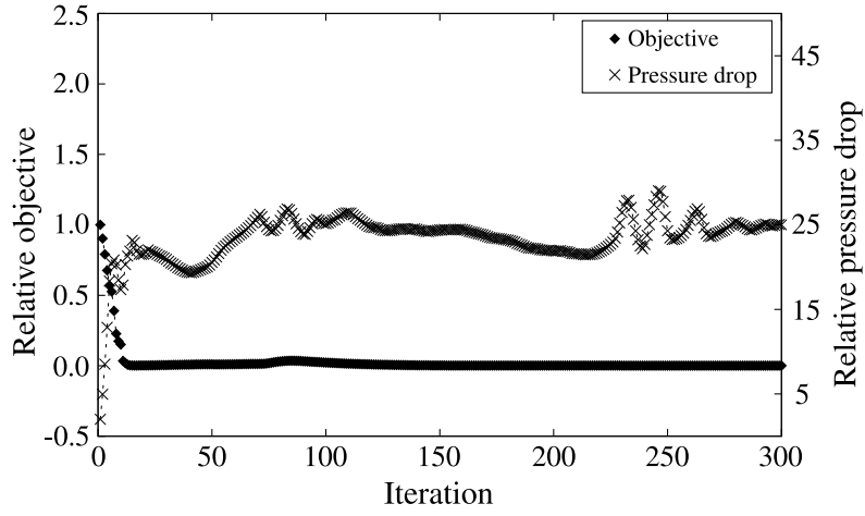
Fig. 5.8 Convergence histories for the extraction efficiency minimization problem in the case of 200\Delta x \times 120\Delta x grids with \eta_{\max} = 25 . Normalized values of objective functional \hat{J}_3 = J_3/J_3^{\text{init}} , with J_3^{\text{init}} representing the initial value of the objective functional. Pressure drop fraction \Delta p/\Delta p^{\text{init}} , with \Delta p representing the current pressure drop.
