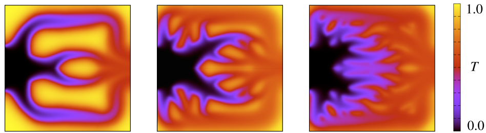
(c) Temperature distributions when \beta_{\max} = 0.1
