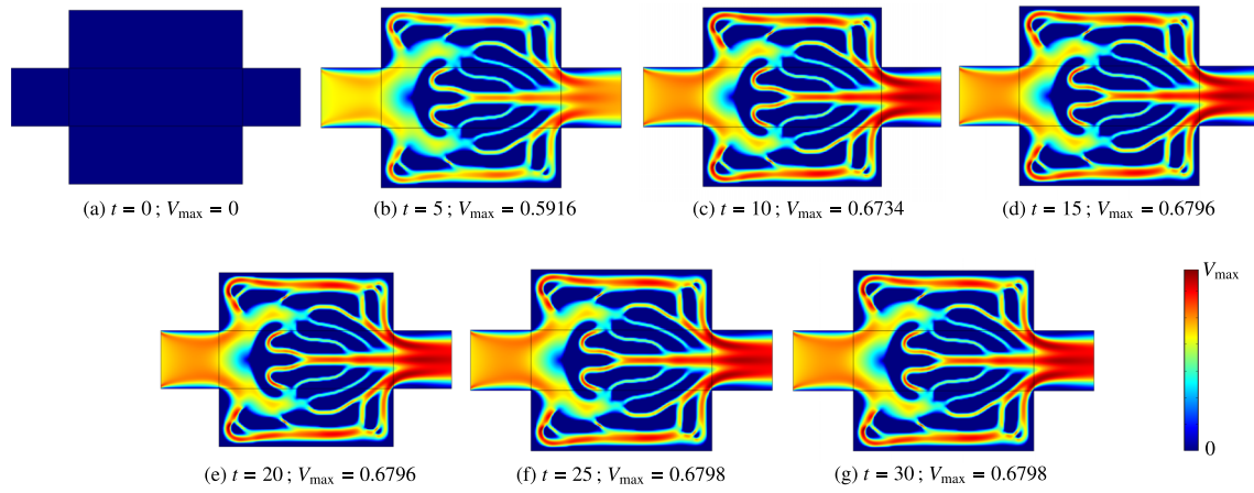
Fig. 2.9 Results of transient flow field calculations to verify that a symmetrical boundary condition and the assumption of a steady-state flow condition are appropriate. The velocity distributions in the optimal configuration for \theta = 500 are shown at each time step. V_{\max} represents the maximum value of velocity magnitude |\mathbf{u}| .
