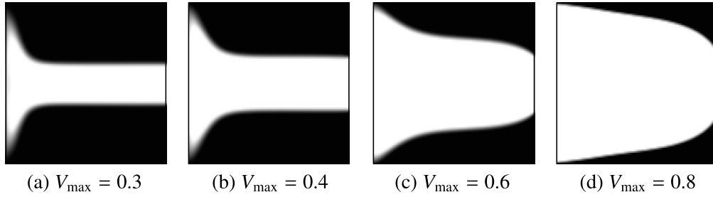
Fig. 3.10 Effect of parameter V_{\max} settings on optimal configurations: (a) V_{\max} = 0.3 , (b) V_{\max} = 0.4 , (c) V_{\max} = 0.6 , (d) V_{\max} = 0.8 .
