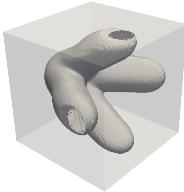
Fig. 3.17 Optimal configurations of the three-dimensional multi-outlets problem, in which the analysis domain is discretized using a 100\Delta x \times 100\Delta x \times 100\Delta x grid. The iso-surface of \gamma = 0.5 is shown as the optimal configuration. The volume constraint is set to V_{\max} = 0.25 .
