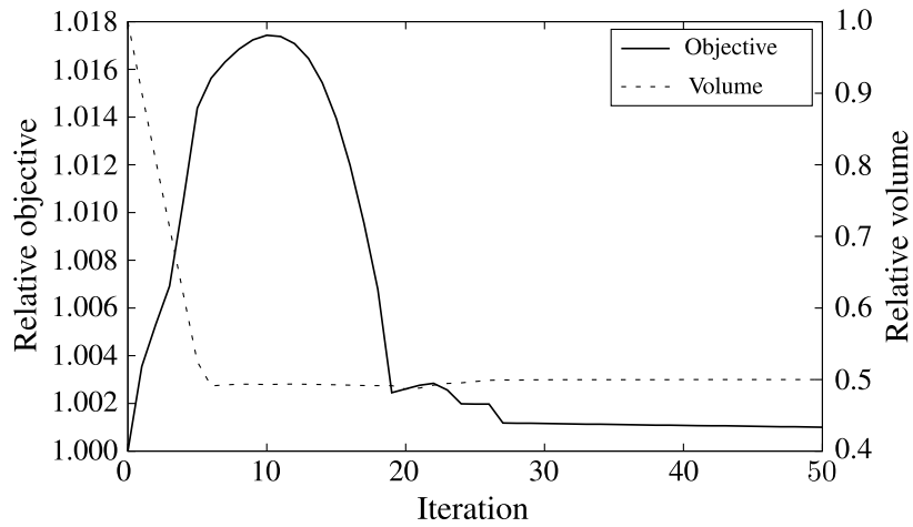
Fig. 3.9 Convergence histories of the relative objective functional and fluid volume. The relative objective functional is defined as \hat{J}_1 = J_1/J_1^{\text{init}} , with J_1^{\text{init}} representing the initial value of the objective functional. The relative fluid volume is defined as \hat{V} = \int_D \gamma d\Omega / \int_D d\Omega . The maximum fluid volume is set to V_{\max} = 0.5 .
