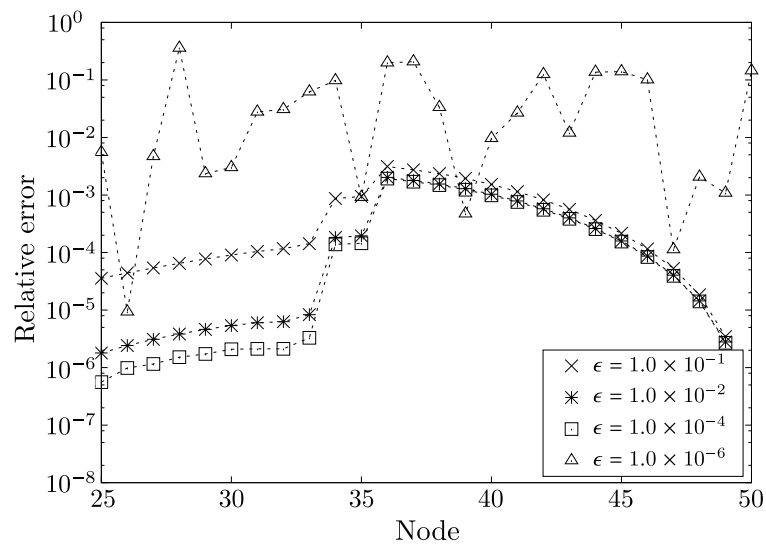
Fig. 3.5 Relative errors of the finite difference approximation with respect to the adjoint sensitivity in the flow resistance minimization problem.
