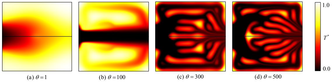
Fig. 2.8 Temperature distribution ( T^* = T/T_{\max} is the regularized temperature, where T_{\max} is the maximum temperature in each optimal configuration, (a) T_{\max} = 0.97 ; (b) T_{\max} = 0.61 ; (c) T_{\max} = 0.21 ; (d) T_{\max} = 0.16 ).
