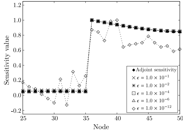
Fig. 4.2 Comparison of the adjoint sensitivity and finite difference approximation in the heat exchange maximization problem using the LBM.
