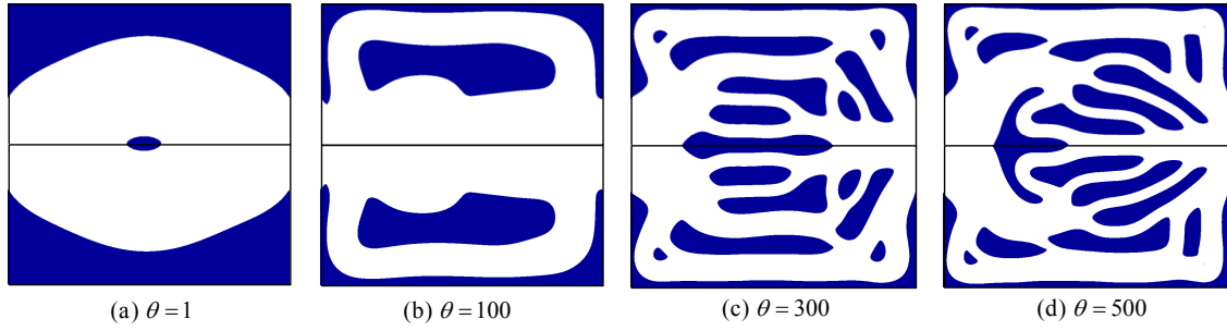
Fig. 2.7 \theta dependency in heat exchange maximization problem (blue, solid domain; white, fluid domain). Reynolds numbers, Re , for each optimal configuration are (a) 1, (b) 70, (c) 170, and (d) 280.
