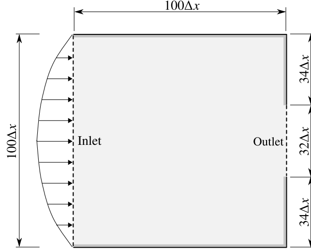
Fig. 3.6 Design settings in the diffuser problem using the LBM.
