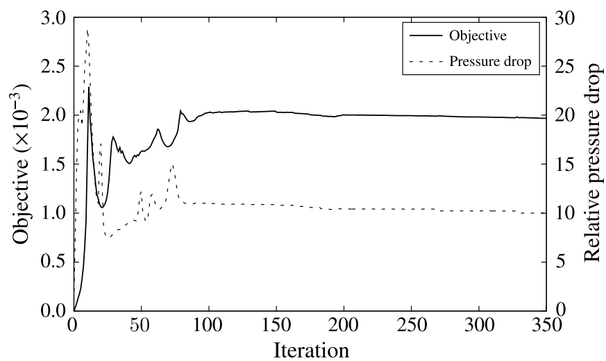
Fig. 4.7 Convergence histories of the objective functional J_2 and the relative pressure drop \Delta p / \Delta p^{\text{init}} , with \Delta p representing the current pressure drop.
