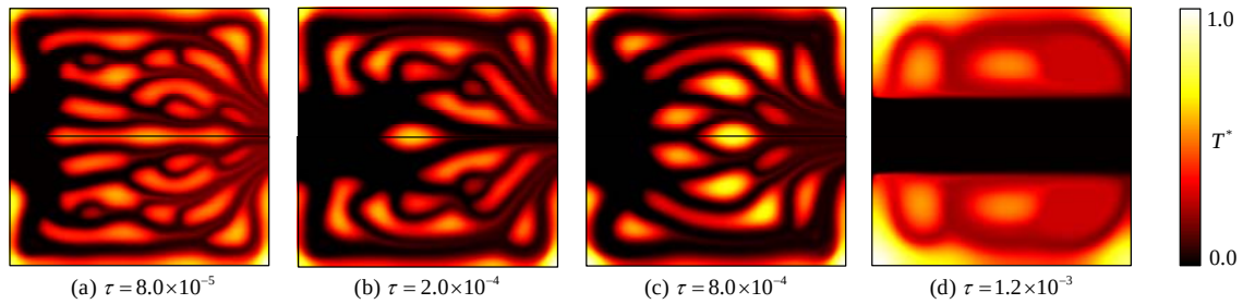
Fig. 2.12 Temperature distribution ( T^* = T/T_{\max} is the regularized temperature, where T_{\max} is the maximum temperature in each optimal configuration, (a) T_{\max} = 0.16 ; (b) T_{\max} = 0.19 ; (c) T_{\max} = 0.19 ; (d) T_{\max} = 0.62 ).
