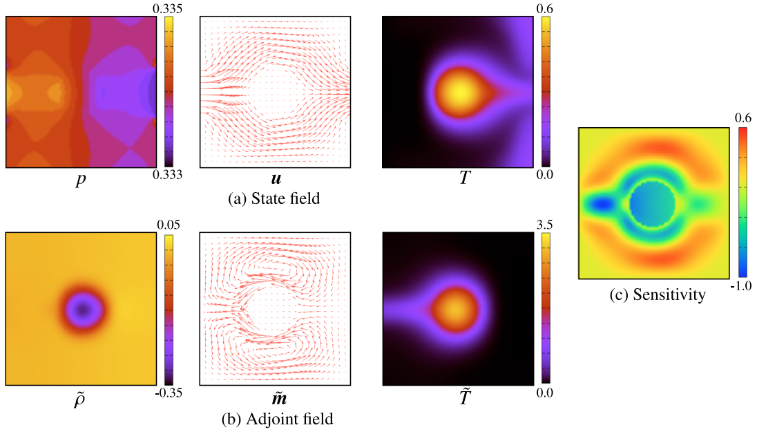
Fig. 4.1 State field ( p , \mathbf{u} , T ), adjoint field ( \rho , \tilde{\mathbf{m}} , \tilde{T} ), and the distribution of adjoint sensitivity in the heat exchange maximization problem using the LBM.
