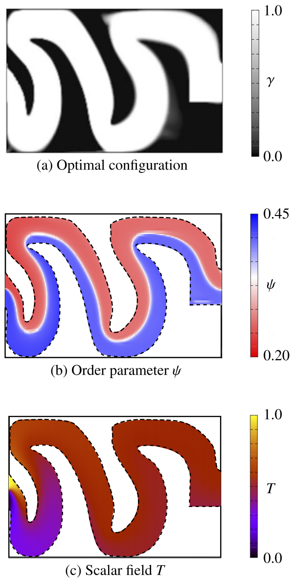
Fig. 5.7 Optimal configuration for the extraction efficiency maximization problem when setting \eta_{\max} = 25 , with the distributions of order parameter \psi and scalar field T .
