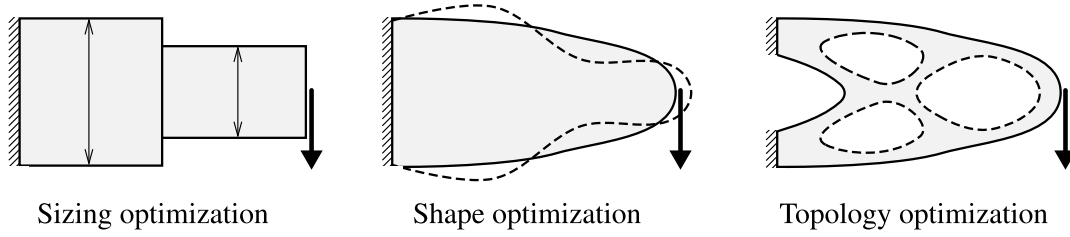
Fig. 1.1 Classification of structural optimization.
