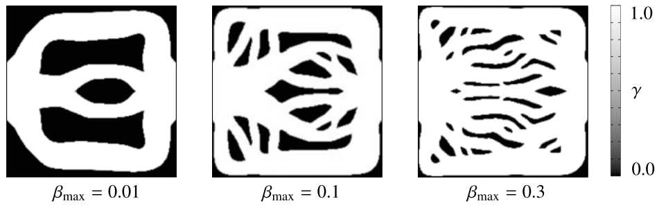
(a) Optimal configurations for different \beta_{\max} values
