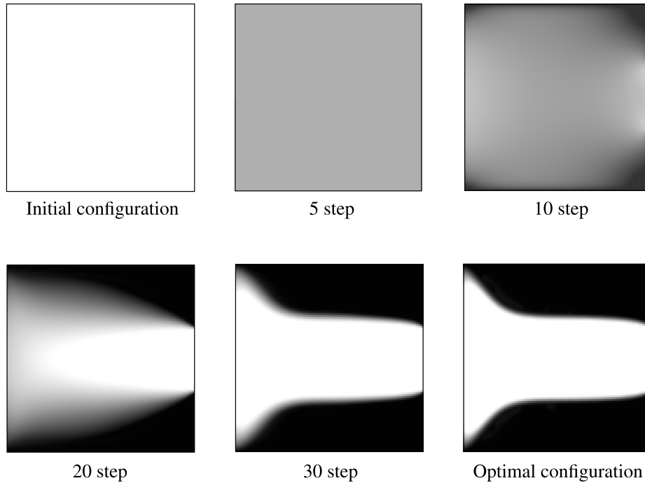
Fig. 3.8 Optimization history of design variable for the diffuser problem using the LBM.
