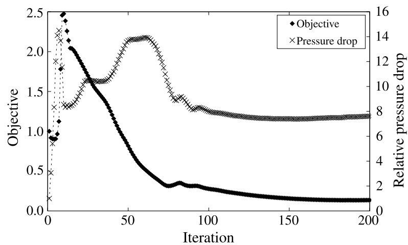
Fig. 5.6 Convergence histories of the relative objective functional \hat{J}_3 = J_3/J_3^{\text{init}} , with J_3^{\text{init}} representing the initial value of the objective function, and the relative pressure drop \Delta p/\Delta p^{\text{init}} , with \Delta p representing the current pressure drop in the extraction efficiency maximization problem.
