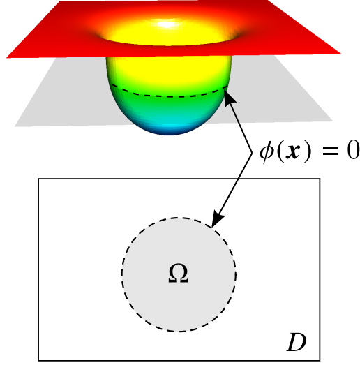
Fig. 2.3 Schematic figure of fixed design domain D and the level set function \phi(\mathbf{x}) based on the piecewise constant function.
