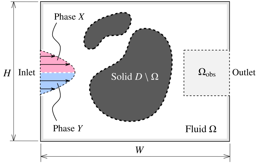
Fig. 5.3 Design domain is composed of the fluid domain \Omega and the solid domain D \setminus \Omega . The objective functional J_3 is evaluated in the observation domain \Omega_{\text{obs}} . The two-phase fluid flows are composed of the phase X and Y that are prescribed on the inlet boundary.
