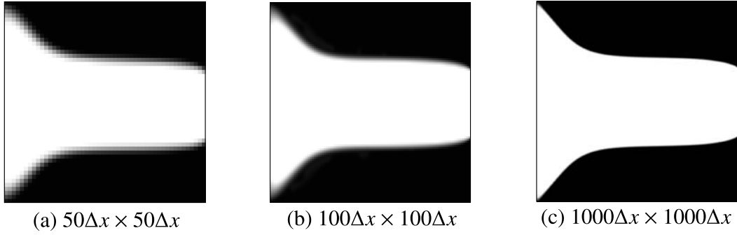
Fig. 3.11 Dependency of optimal configurations on grid size in the diffuser problem using the LBM: (a) 50\Delta x \times 50\Delta x , (b) 100\Delta x \times 100\Delta x , (c) 1000\Delta x \times 1000\Delta x .
