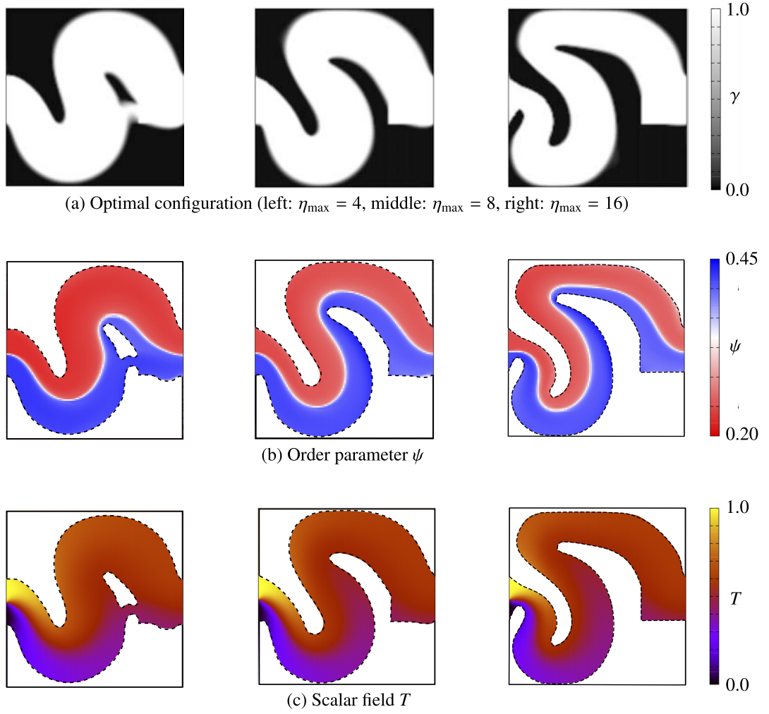
Fig. 5.4 Optimal configurations in the extraction efficiency maximization problem, with the distributions of order parameter \psi and scalar field T in the different settings of pressure drop coefficient: \eta_{\max} = 4 (left side figures); \eta_{\max} = 8 (middle figures); \eta_{\max} = 16 (right side figures).
