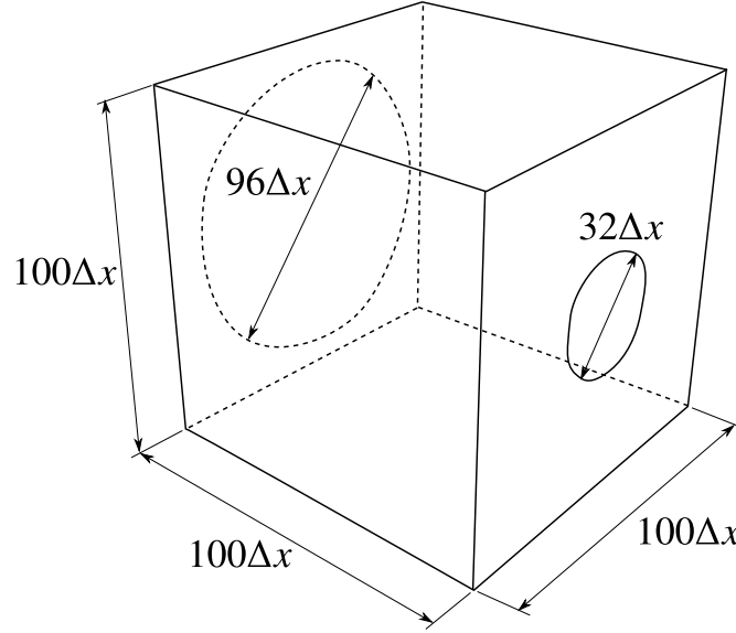
Fig. 3.14 Design settings for the three-dimensional diffuser problem. The analysis domain is discretized using a 100\Delta x \times 100\Delta x \times 100\Delta x grid.
