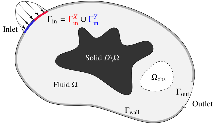
Fig. 5.2 Schematic figure of fixed design domain D composed of the fluid domain \Omega , solid domain D \setminus \Omega and observation domain \Omega_{\text{obs}} . The boundary of fixed design domain is defined as \Gamma = \Gamma_{\text{in}} \cup \Gamma_{\text{out}} \cup \Gamma_{\text{wall}} with \Gamma_{\text{in}} \cap \Gamma_{\text{out}} \cap \Gamma_{\text{wall}} = \emptyset .
