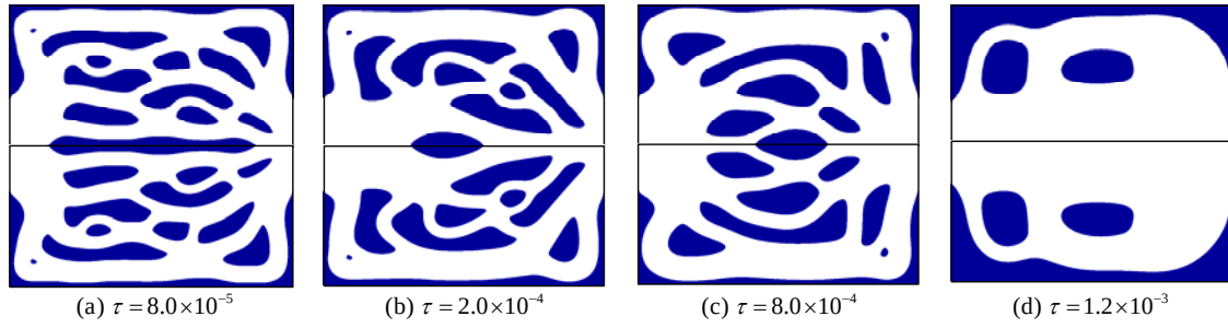
Fig. 2.11 Regularization parameter dependency in heat exchange maximization problem (blue, solid domain; white, fluid domain). Reynolds numbers, Re , for each optimal configuration are (a) 210, (b) 270, (c) 280, and (d) 800.
