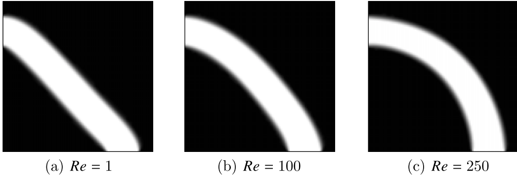
Fig. 3.13 Dependency of optimal configurations on the value of Reynolds number in the pipe bend problem using the LBM: (a) Re = 1 , (b) Re = 100 , (c) Re = 250 .
