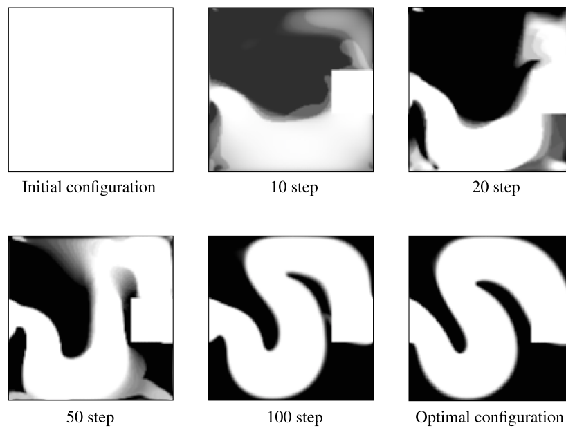
Fig. 5.5 Optimization history of design variable for the extraction efficiency maximization problem.
