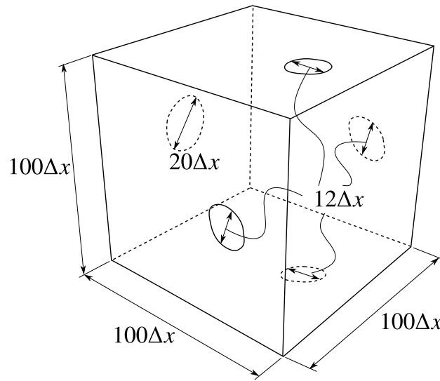
Fig. 3.16 Design settings in the three-dimensional multi-outlets problem. The analysis domain is discretized using a 100\Delta x \times 100\Delta x \times 100\Delta x grid.
