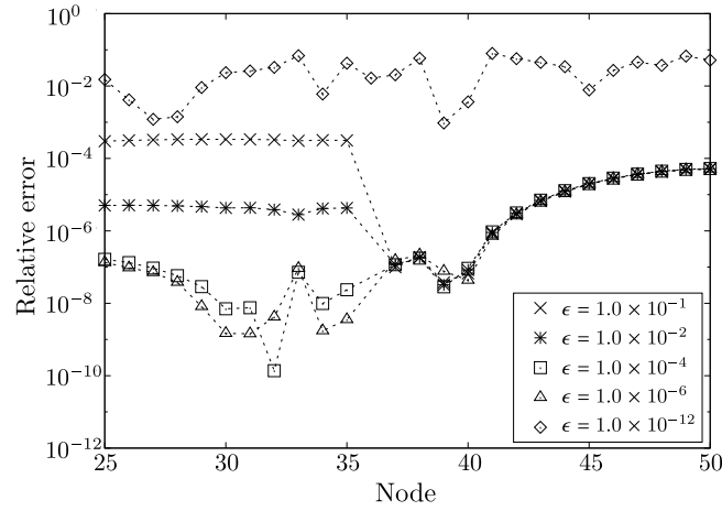
Fig. 4.3 Relative errors of the finite difference sensitivities with respect to the adjoint sensitivity in the heat exchange maximization problem using the LBM.
