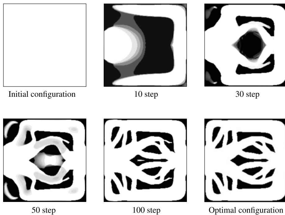
Fig. 4.6 Optimization history of design variable for the heat exchange maximization problem.
