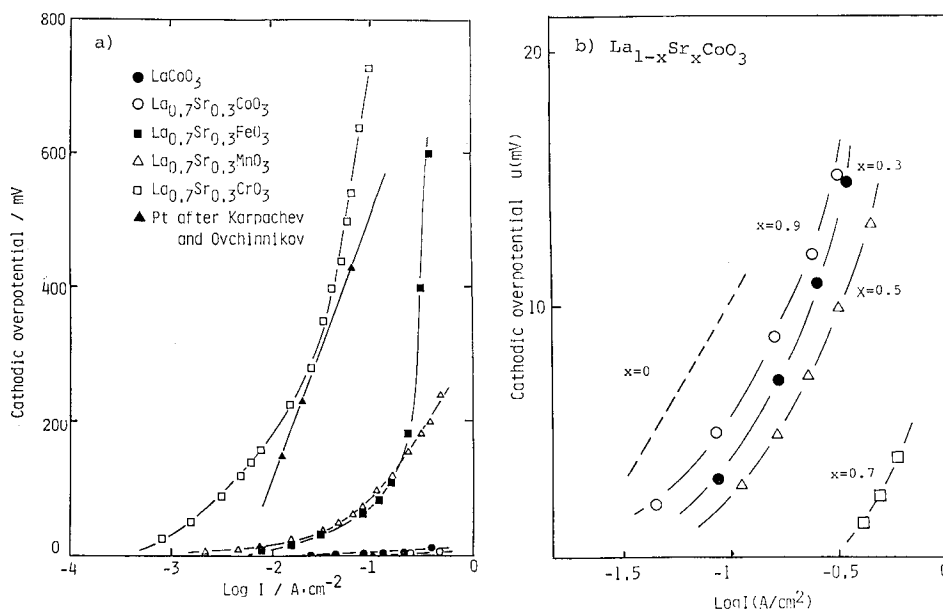
Fig. 5. Cathodic polarization curves at 800°C for the sputtered \text{La}_{1-x}\text{Sr}_x\text{MO}_{3-z} electrodes.
