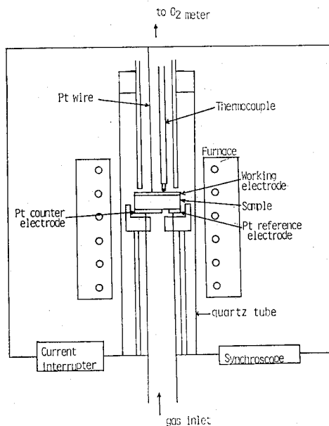
Fig. 1. Experimental cell.
