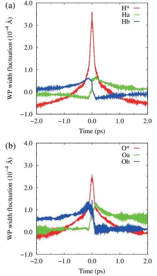
FIG. 8: Averaged trajectories of the wave packet (WP) width fluctuations of (a) H atoms and (b) O atoms in the OH-SQW model. The WP width fluctuation is defined by the difference from the statistical average.
