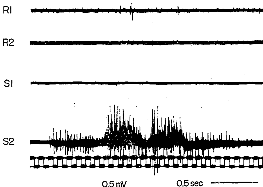
Fig. 1. Discharges of impulses in the femur muscle caused by direct application of 2.8 \times 10^{-5}M DDT to the exposed thoracic ganglia in DDT-resistant ( R bwb ; ocra ; ar ; ac ) strain and in susceptible Lab strain of houseflies. R: resistant strain. S: susceptible strain. 1: before application of DDT. 2: 9 minutes after DDT.
