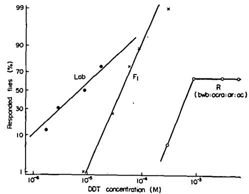
Fig. 2. Dosage-nerve sensitivity relationships to DDT in susceptible Lab strain ( \bullet ), in resistant marker strain ( \circ ), and in the F 1 hybrid ( \times ). Nerve sensitivity is expressed as the percentage of the "responded" flies in a population tested.
