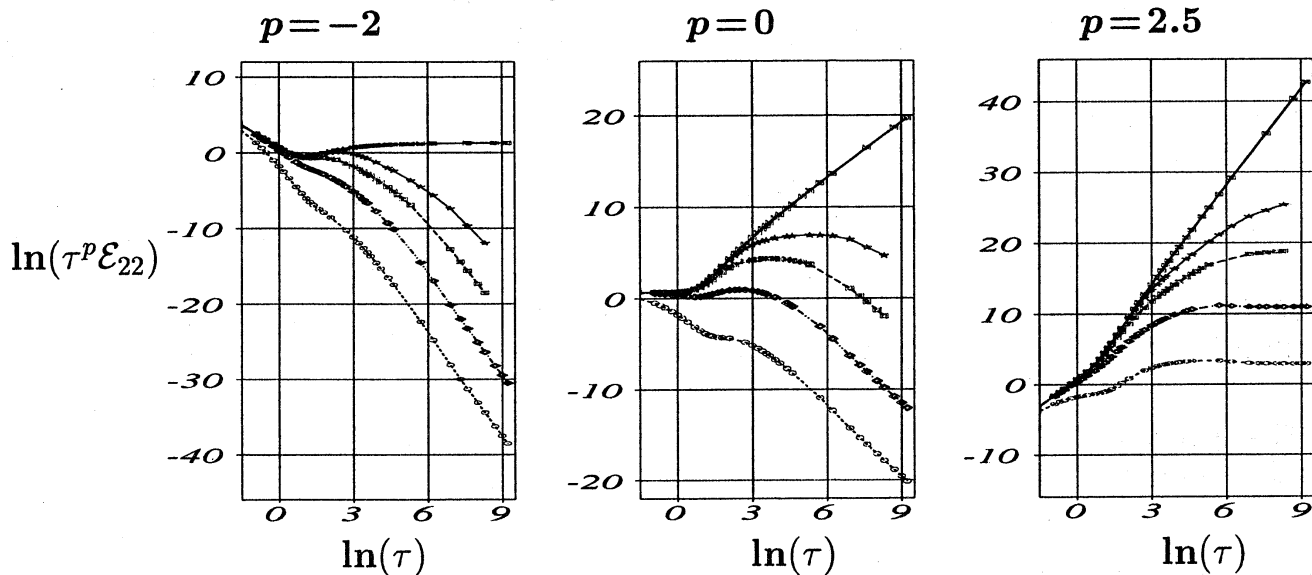
Figure 6: Spanwise “enstrophy tensor” compensated by different power-laws, \mathcal{E}_{22}(\tau) \tau^{-p} . From topmost curve downward, on each plot, N = 0, 10^{-3}, 10^{-2}, 10^{-1}, 1 .
