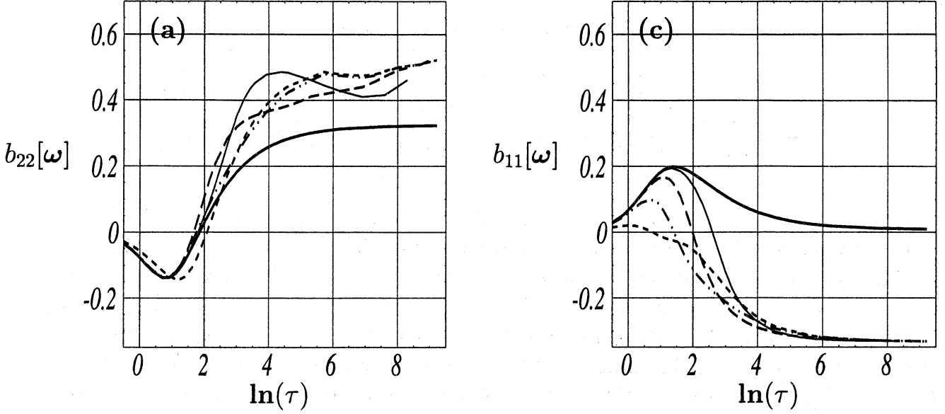
Figure 8: SSRDT for vorticity anisotropy tensor components b_{ij}[\omega] .
