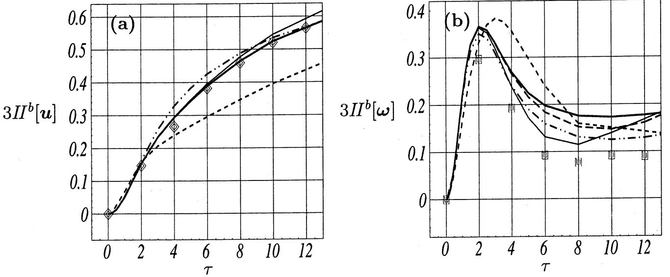
Figure 3: Evolution of the 2nd invariant of the anisotropy tensor for (a) the velocity and (b) the vorticity field. Symbols denote DNS data [8]. Lines connect SSRDT data sequences for N=0 (—), 10^{-3} (— — —), 10^{-2} (— · — · —), 10^{-1} (— · — · —), 1 (· · · · ·).
