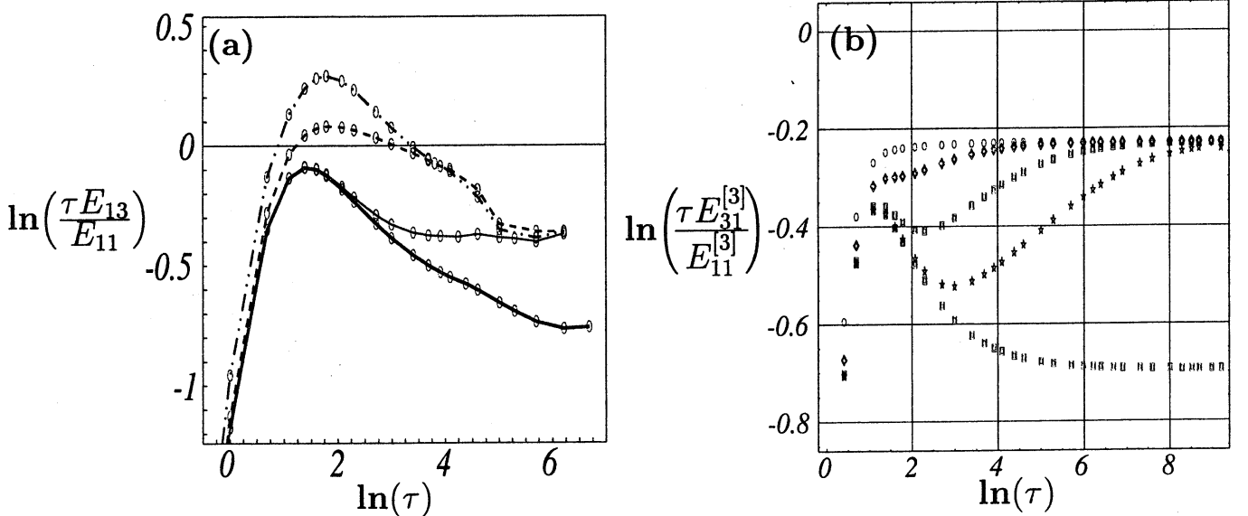
Figure 5: Compensated (a) single-point and (b) two-point ratios of Reynolds stress to streamwise (dominant) componental energy. From lowest curve up, (b): N = 0, 10^{-3}, 10^{-2}, 10^{-1}, 1 ; (a): 10^{-3} not shown. Asymptotes \tau \text{ const.} have \text{const.} < 1 closer to 1 in the viscous case.
