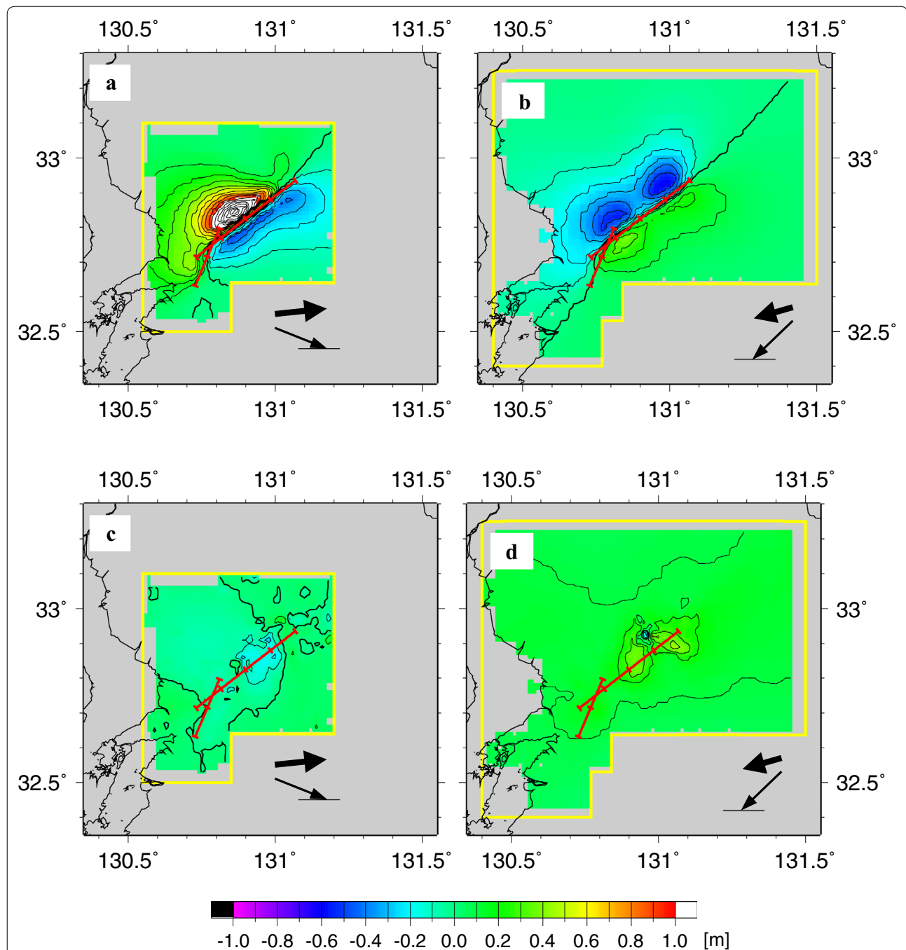
Fig. 5 Synthetic displacement and residual. a, b Synthetic LOS displacement for the right- (path 135–650; a ) and left (path 124–700; b )-looking images, computed from the optimal slip model shown in Fig. 4. c, d Residual LOS displacement for the right- ( c ) and left ( d )-looking images, generated by subtracting the model LOS displacement ( a, b ) from the observed data (Fig. 2a, b). The red lines with ticks show the model fault traces for the inversion analysis. The thick arrow shows the approximate direction of LOS vectors projected onto the horizontal plane. The thin arrow with a horizontal short line shows the approximate incidence angle. The contour interval in LOS displacement is 10 cm
