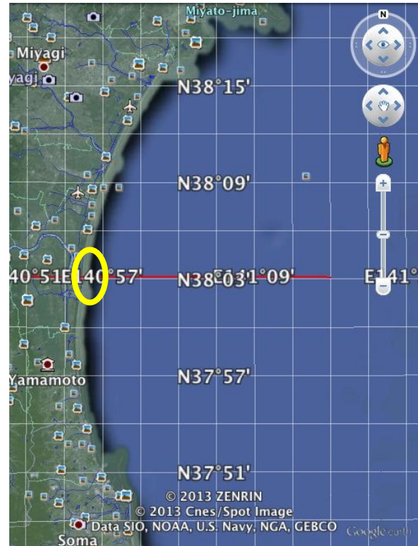
Fig 4b Domain of the model (Google Earth, 11 th of February 2013)
