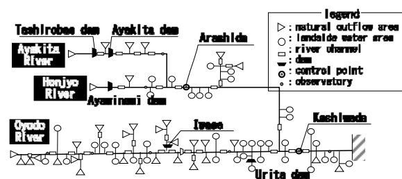
Fig.6 Calculation model for storage function method
