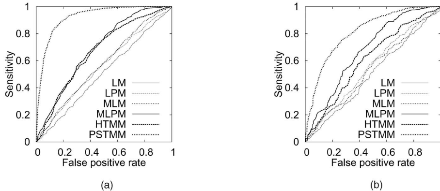
Fig. 8. ROC curves for (a) N-Glycans and (b) O-Glycans.
