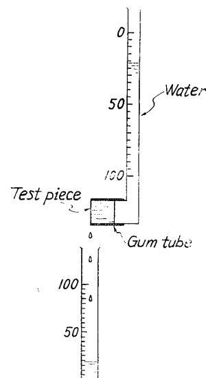
Fig. 1. Apparatus for measuring water permeability of wood.
