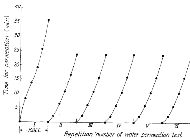
Fig. 2-1. Relation between water permeation and time. When the test piece was dried in advance, the first permeation needs somewhat longer time than the subsequent one.
