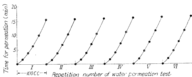
Fig. 2-2. Relation between water permeation and time. When the test piece was wetted with water or alcohol in advance, the time elapsed for water permeation was almost alike in every time of the repeated tests.
