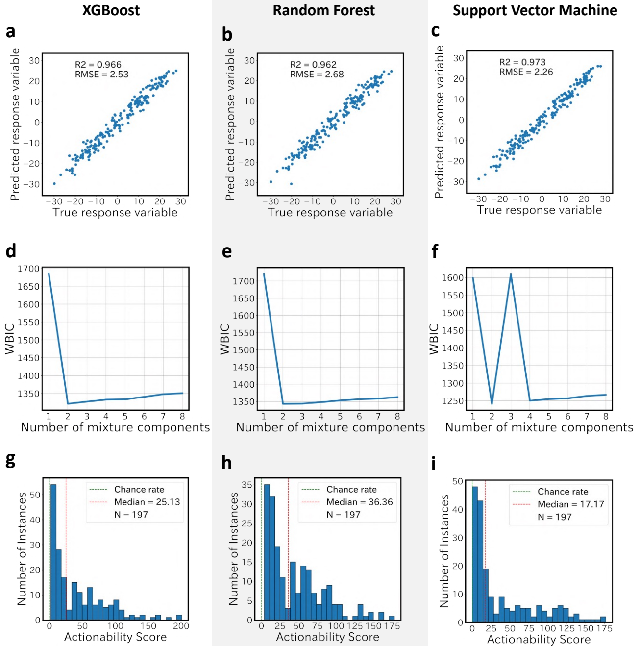
Supplementary Figure 12. Results of the proposed framework on five-dimensional (5D) synthetic dataset. The results of applying our framework to prediction models based on nonlinear machine learning (ML) algorithms are shown: XGBoost ( a, d, g ), random forest ( b, e, h ), and support vector machine ( c, f, i ). a–c Plots for prediction vs. true response variable. d–f Widely applicable Bayesian information criterion (WBIC) values of stochastic surrogate models with 1–8 mixture components. g–i Histogram of actionability scores with intervention variables based on data-driven selection at different instances. An actionability score of zero indicates that the actionability of the optimal path is equivalent to that of the baseline path.
