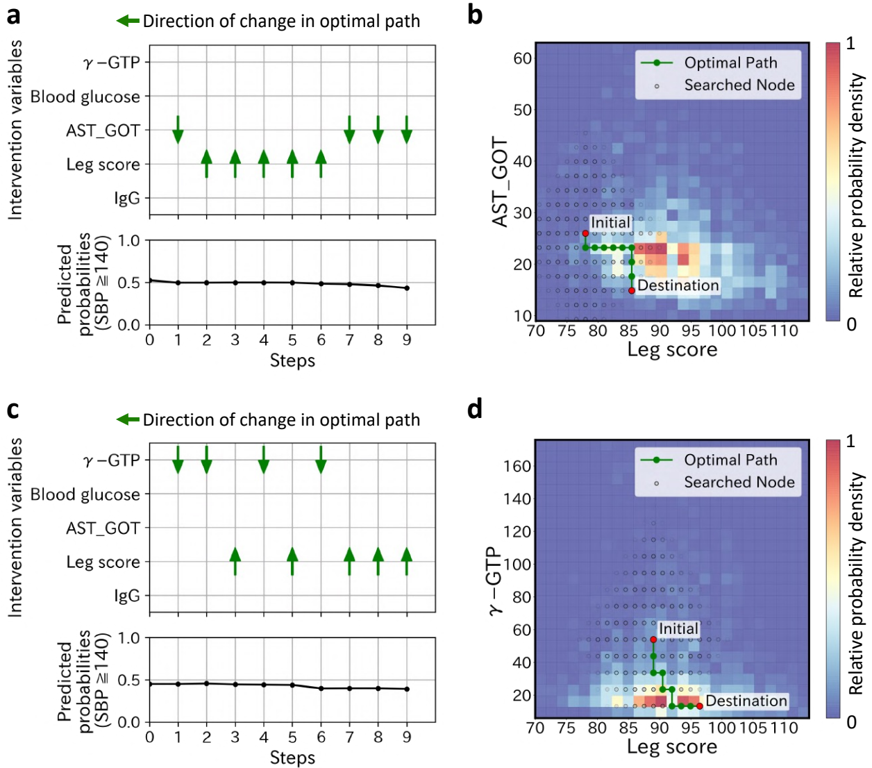
Supplementary Figure 24. Examples of personal actionable paths for treatment in hypertension risk classification task using random forest (RF). The optimal paths for improving the response variable predicted by the RF model are represented for the same instances selected on the application to XGBoost: instance 7 ( a, b ) and instance 8 ( c, d ). a, c The orders of changes in the explanatory variables in the optimal path and the accompanying changes in the predicted values. In the transition steps, the upward or downward arrow represents a unit increase or decrease in the explanatory variable, respectively. b, d 2D plots of the path. The 2D plots are shown regarding the two influential variables in the optimal path: aspartate transaminase (AST [GOT]) and leg score ( b ), and gamma glutamyl transferase (g-GTP) and leg score ( d ). In the heatmaps, the probability density of the actual data, normalized by the panel with the maximum number of data, is expressed.
