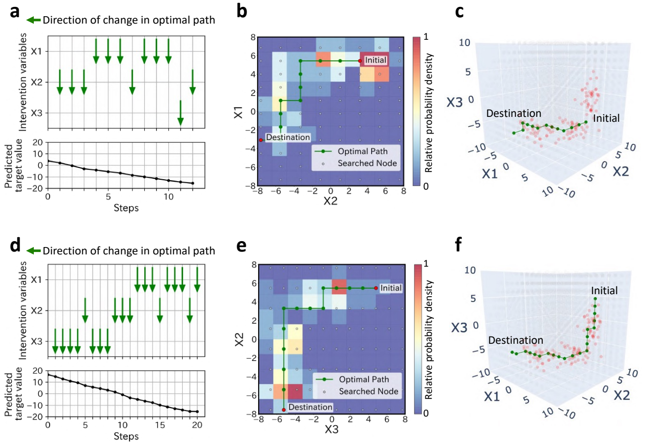
Supplementary Figure 11. Examples of actionable paths planned using support vector machine (SVM) model on three-dimensional (3D) synthetic dataset. The optimal paths for improving the response variable predicted by the SVM model are represented for the same instances selected on the application to XGBoost: instance A ( a–c ) and instance B ( d–f ). a, d The orders of changes in the explanatory variables in the optimal path and the accompanying changes in the predicted values. In the transition steps, the upward or downward arrow represents a unit increase or decrease in the explanatory variable, respectively. b, e 2D plots of the path. The 2D plots are shown regarding the selected two variables: X1 and X2 ( b ), and X2 and X3 ( e ). In the heatmaps, the probability density of the actual data, normalized by the panel with the maximum number of data, is expressed. c, f 3D plots of the path.
