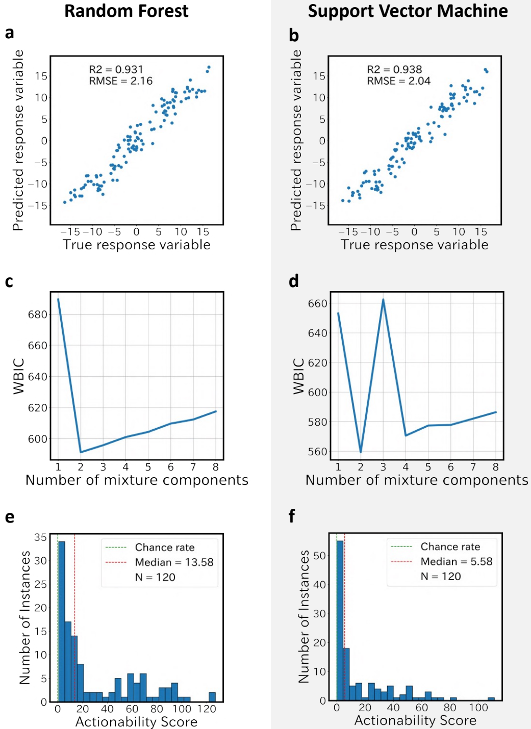
Supplementary Figure 9. Results of the proposed framework on three-dimensional (3D) synthetic dataset using different machine learning (ML) algorithms. The results of applying our framework to prediction models based on nonlinear ML algorithms other than XGBoost are shown: random forest ( a , c , e ) and support vector machine ( b , d , f ). a , b Plots for prediction vs. true response variable. c , d Widely applicable Bayesian information criterion (WBIC) values of stochastic surrogate models with 1–8 mixture components. e , f Histogram of actionability scores with intervention variables based on data-driven selection at different instances. An actionability score of zero indicates that the actionability of the optimal path is equivalent to that of the baseline path.
