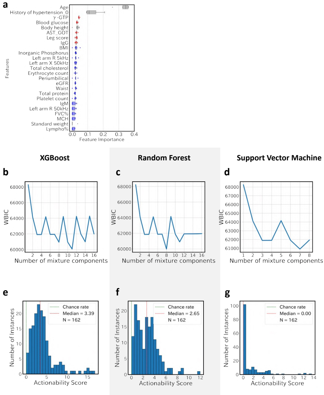
Supplementary Figure 22. Results of the proposed framework on hypertension risk classification task. a
