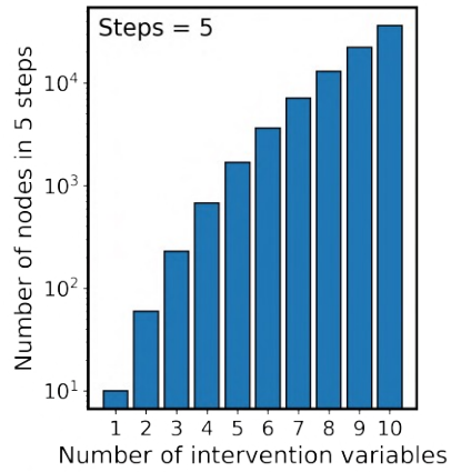
Supplementary Figure 31. Number of nodes within certain number of steps without detours. The number of nodes within 5, 10, or 15 steps are shown. The vertical axis is represented on a logarithmic scale. As the intervention variable increases, the number of nodes increases exponentially, which causes multistep path planning difficult.
