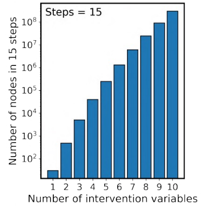
Supplementary Figure 31. Number of nodes within certain number of steps without detours. The number of nodes within 5, 10, or 15 steps are shown. The vertical axis is represented on a logarithmic scale. As the intervention variable increases, the number of nodes increases exponentially, which causes multistep path planning difficult.
