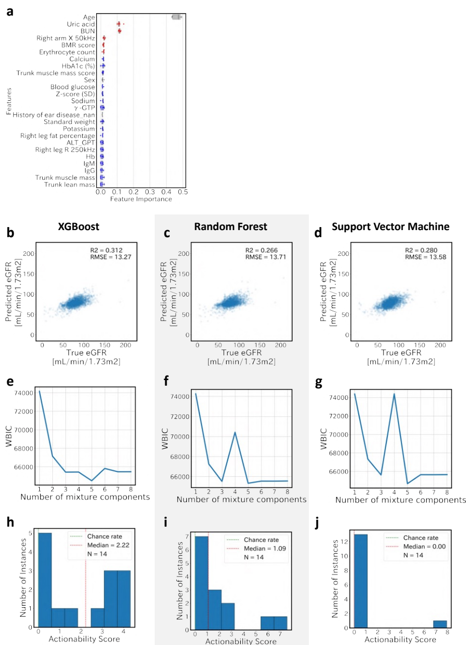
Supplementary Figure 26. Results of the proposed framework estimated glomerular filtration rate (eGFR) regression task. a Feature importance. These 25 features were selected by recursive feature elimination (RFE). RFE was performed with five-fold cross-validation, and the feature importance when 25 variables remained is shown for each fold ( n = 5 ). The plot color represents the following: red: intervention variables, gray: variables which cannot be intervened, and blue: other variables. In box-plot, center line represents median; box limits, upper and lower quartiles; whiskers, 1.5x interquartile range. Details of features are described in Supplementary Data 1. b–j The results of applying our framework to prediction models based on nonlinear machine learning (ML) algorithms: XGBoost ( b , e , h ), random forest ( c , f , i ), and support vector machine ( d , g , j ). b–d Plots for prediction vs. true response variable. e–g Widely applicable Bayesian information criterion (WBIC) values of stochastic surrogate models with 1–8 mixture components. h–j Histogram of actionability scores. An actionability score of zero indicates that the actionability of the optimal path is equivalent to that of the baseline path.
