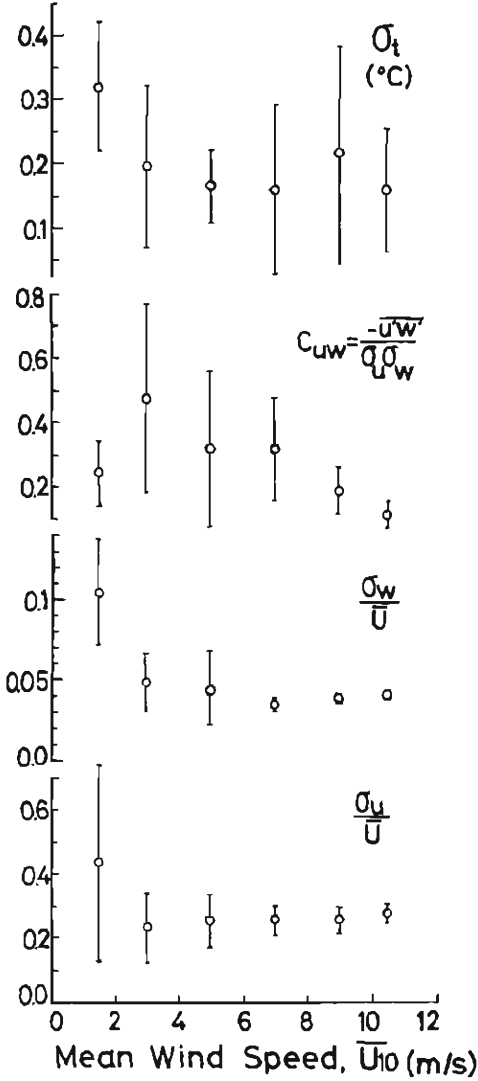
Fig. 5. The standard deviation of temperature, the correlation coefficient between u and w, intensity of turbulence of the vertical component and that of horizontal component from the top to the bottom as functions of wind speed at 10 m (Biwako, 1972).
