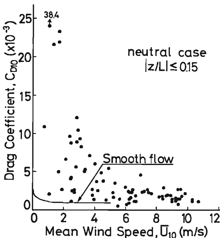
Fig. 3. Neutral drag coefficient as a function of wind speed at 10 m as observed over the shallow inland water surface (Biwako, 1972).
