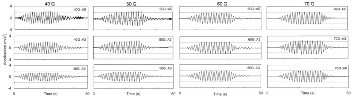
Figure 6. Time histories of input (A0) and response (A3 and A5) acceleration of Cases 40 G to 70G.
