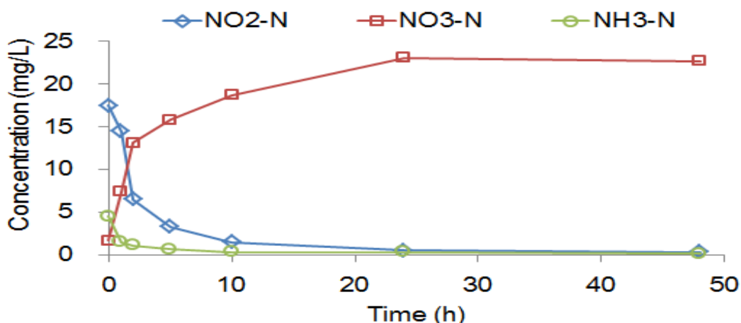
Figure 6.6 Profile of NO 2 -N, NO 3 -N and NH 3 -N concentration under nitrite oxidizing conditions
