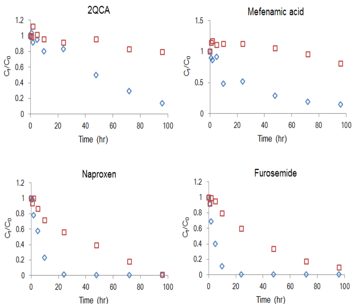
Figure 6.5 Changes of relative concentration of target compounds with and without AOB inhibition
