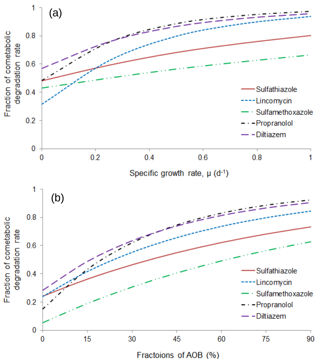
Figure 7.6 Prediction of cometabolic degradation rate for target compounds depending on the variations of (a) specific growth rate, \mu and (b) fractions of AOB
