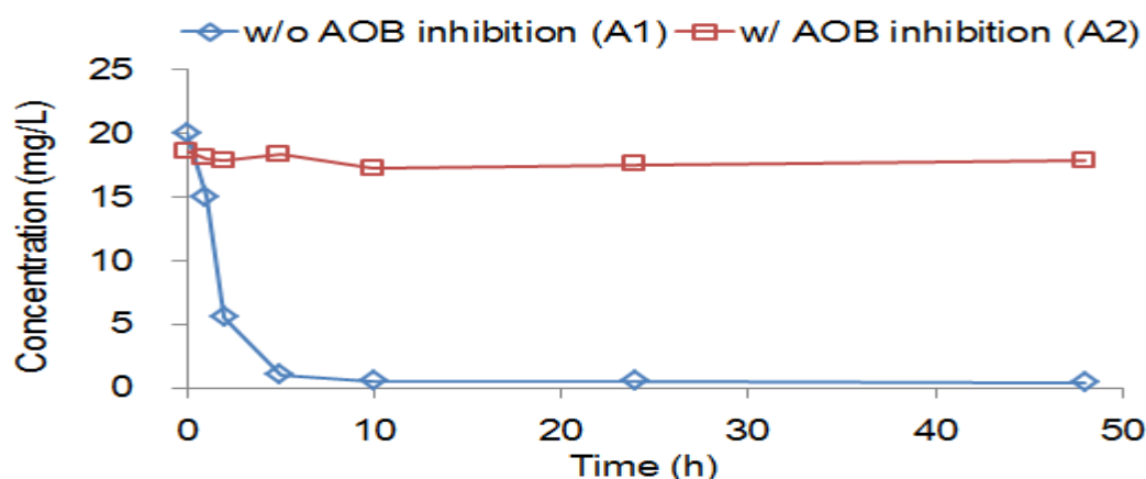
Figure 6.4 Profile of \text{NH}_3\text{-N} concentration with and without AOB inhibition
