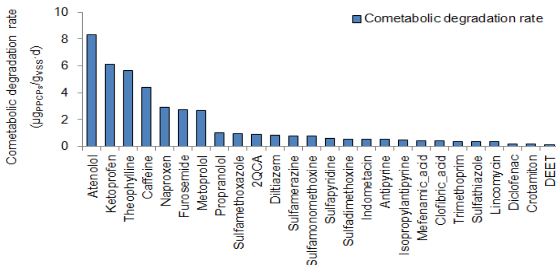
Figure 6.7 Cometabolic degradation rates of PPCPs
