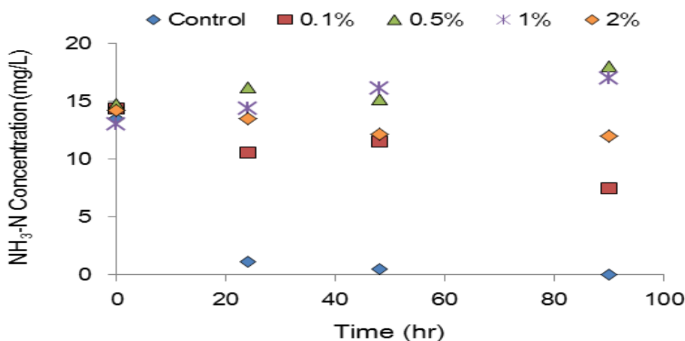
Figure 5.1 Variation of \text{NH}_3\text{-N} concentrations as a function of \text{NaN}_3 concentration
