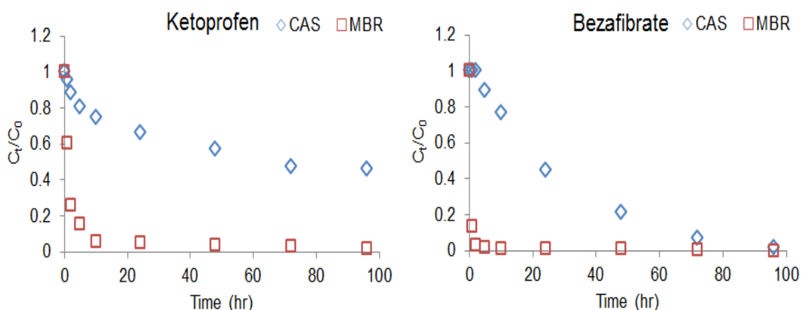
Figure 5.2 Changes of relative concentration of the compounds showing high removal in MBR and high/moderate removal in CAS
