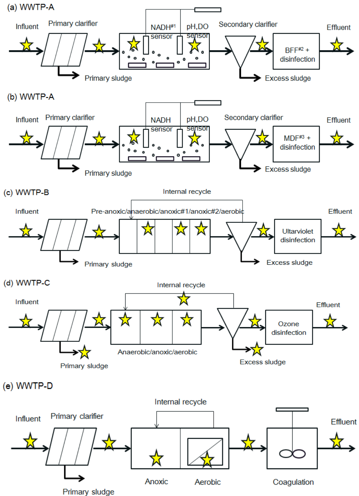
Figure 3.1 Process diagram and sampling points of WWTPs
