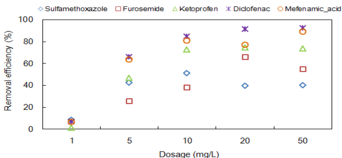
Figure 4.8 Removal efficiency by PAC
