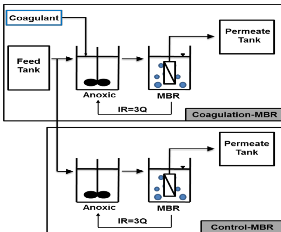
Figure 4.1 Schematic diagrams of coagulation-MBR and control-MBR in stage 3
