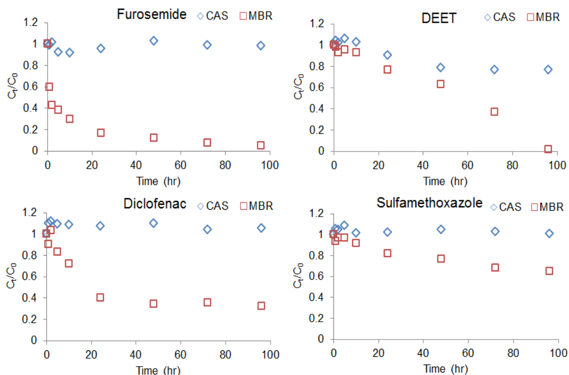
Figure 5.3 Changes of relative concentration of the compounds showing moderate removal in MBR and poor removal in CAS
