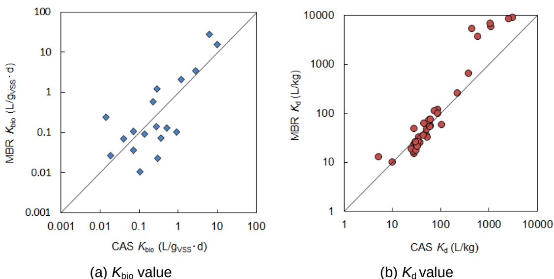
Figure 5.5 Comparison of K_{bio} and K_d values between MBR and CAS
