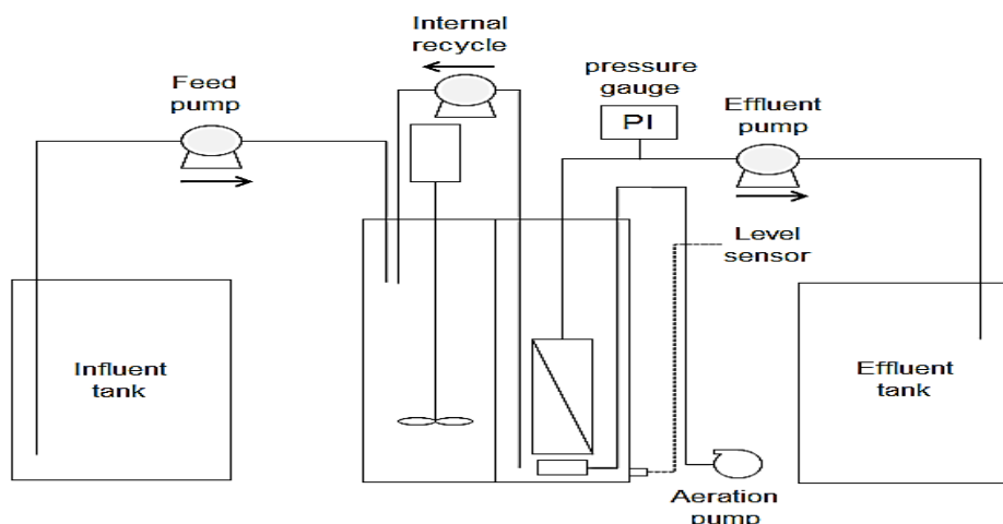
Figure 3.2 Schematic diagram of lab-scale MBR
