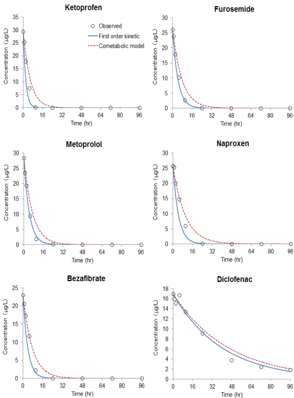
Figure 7.4 Comparison between observed and predicted removal for the compounds showing a high goodness of fit in pseudo first-order model
