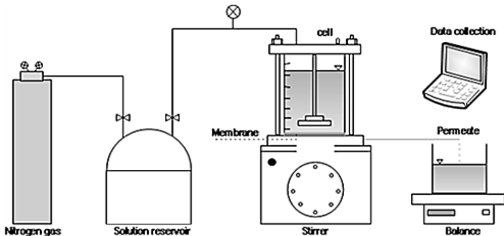
Figure 4.2 Schematic diagram of filtration experiment
