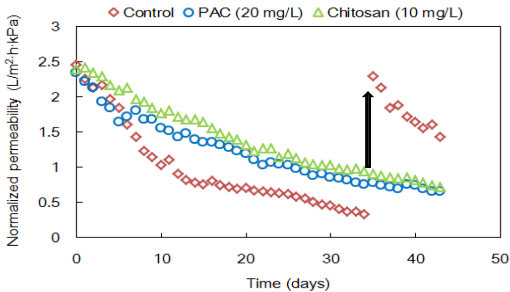
Figure 4.6 Normalized permeability by coagulation
