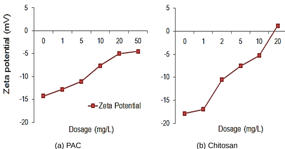
Figure 4.5 The change of zeta potential
