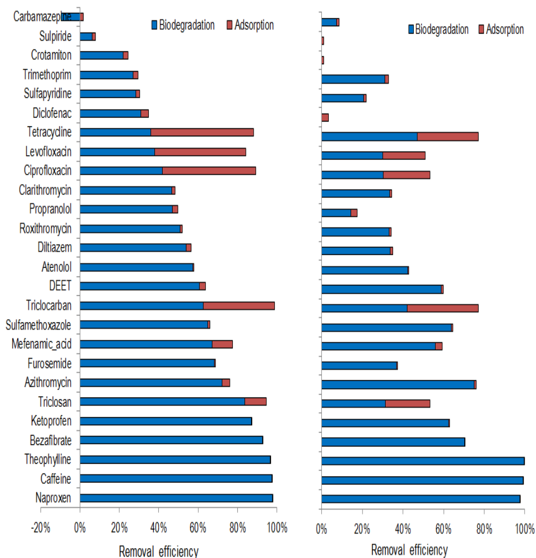
Figure 3.10 Mass balance of lab-scale MBR (left) and A2O process (WWTP-C, right)
