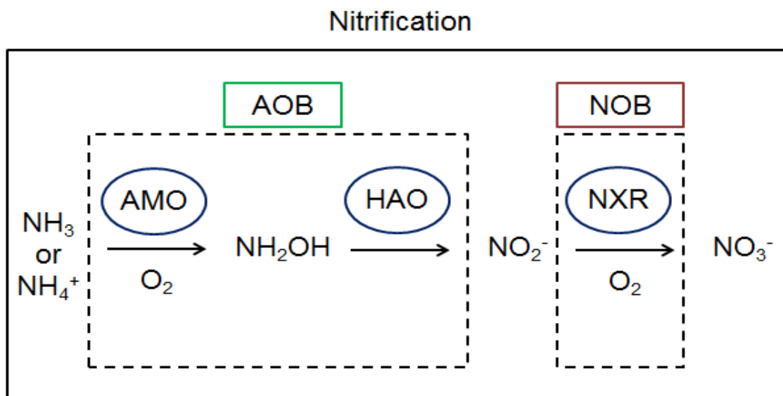
Figure 6.1 Schematic diagram of nitrification process by AOB and NOB
