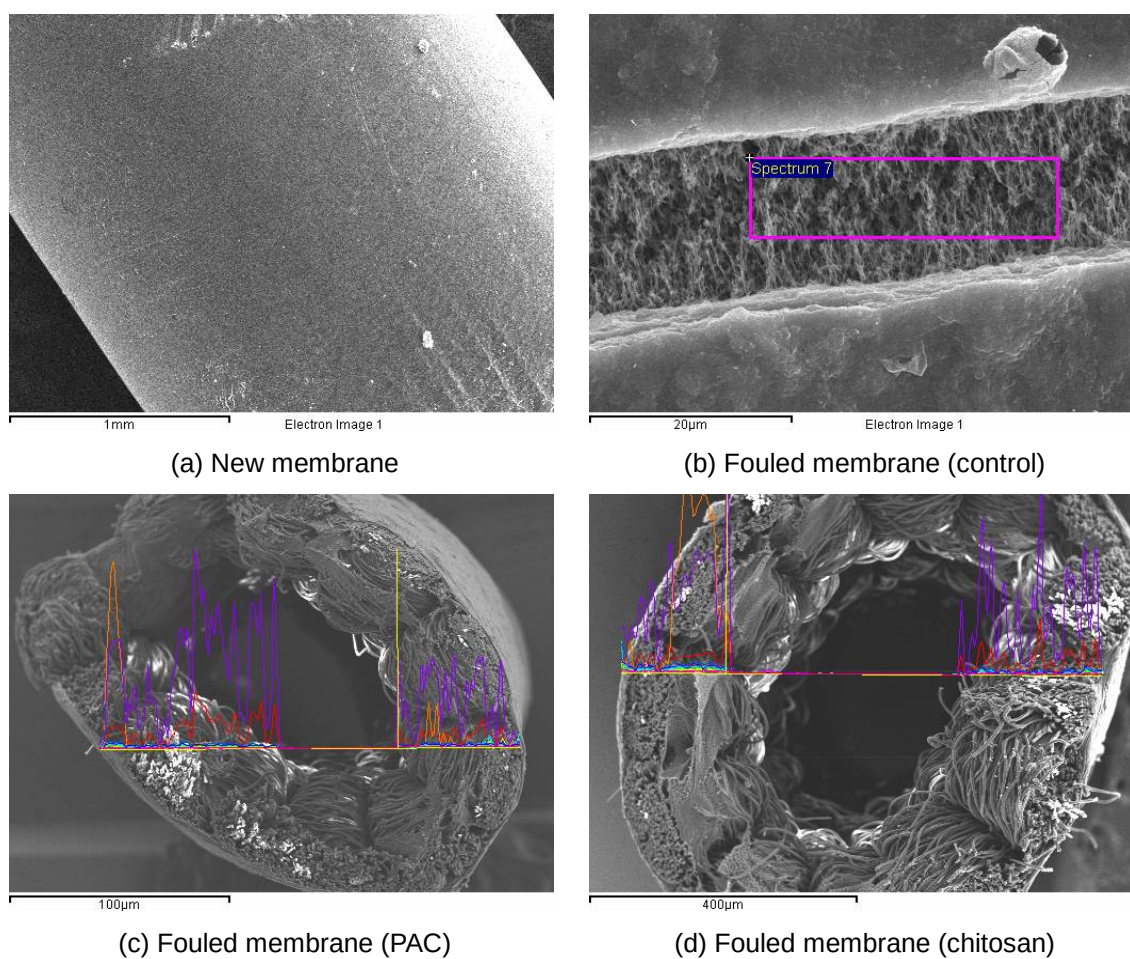
Figure 4.7 The images of SEM analysis
