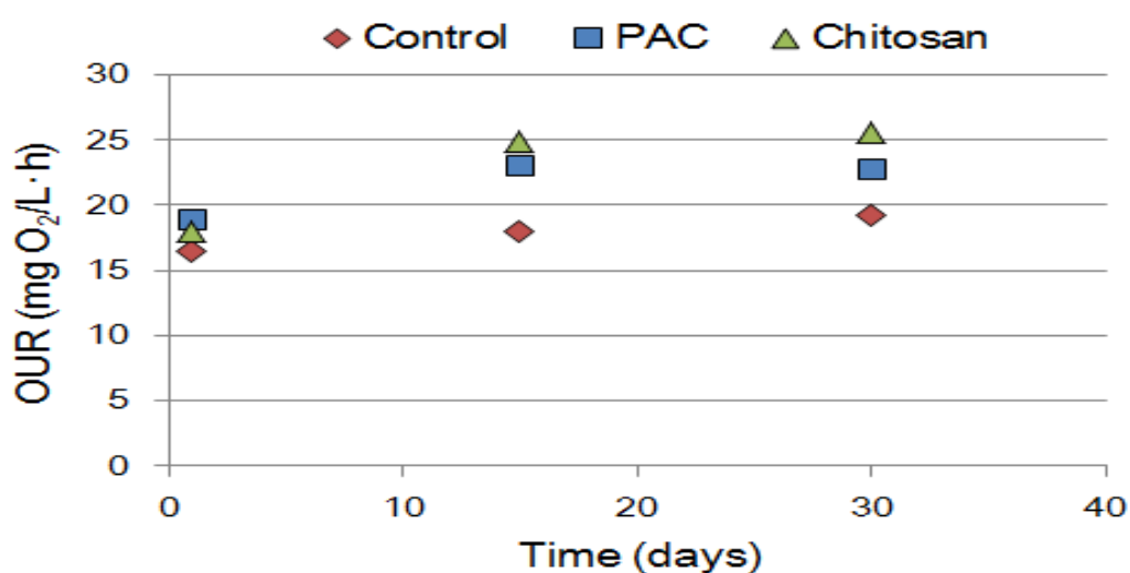
Figure 4.11 OUR profile of control, PAC and chitosan
