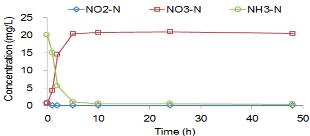
Figure 6.3 Profile of NO 2 -N, NO 3 -N and NH 3 -N concentration with no AOB inhibition
