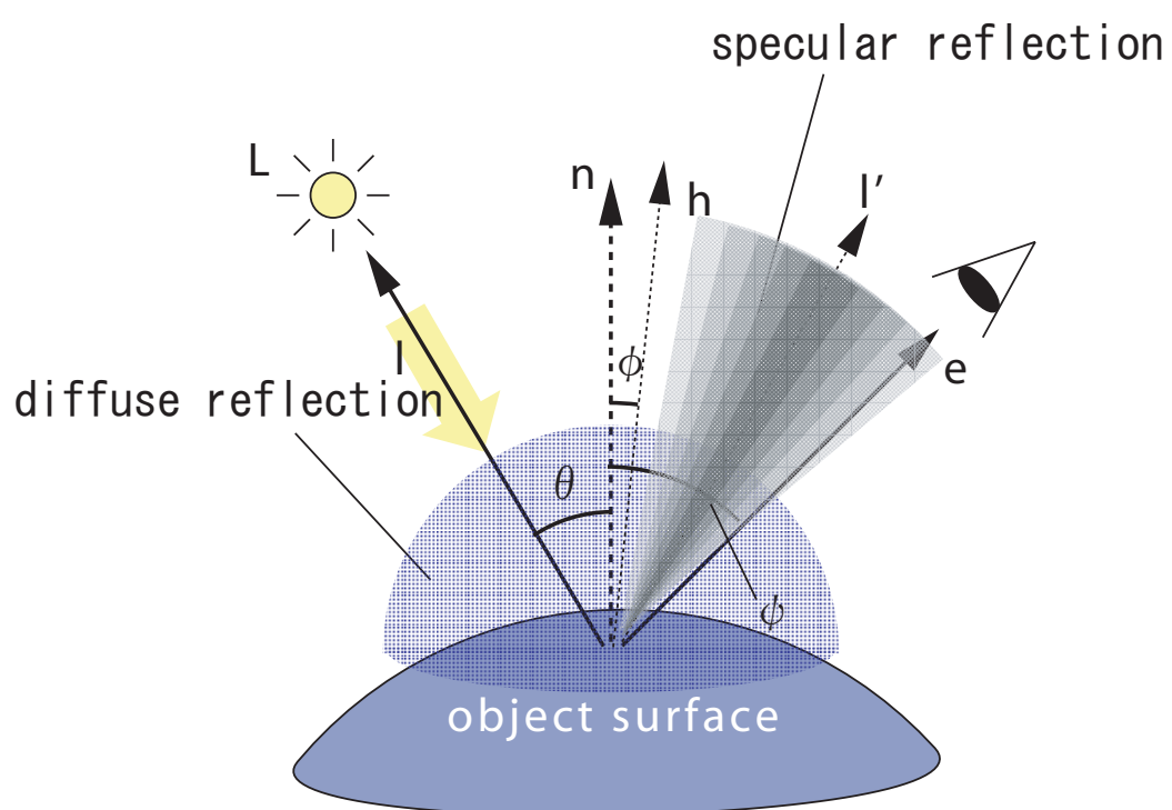
Figure 2.3: Light Reflection.
