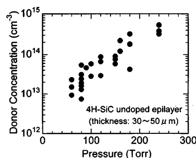
FIG. 1. Pressure dependence of donor concentration for unintentionally doped epilayers. The donor concentration was determined by C-V characteristics of 1.5 mm \phi Ni/4H-SiC Schottky structure processed on 30–50 \mu\text{m} thick epilayers grown on highly doped n -type substrates.
