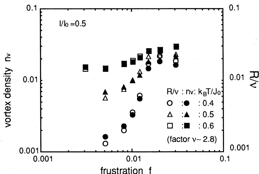
図 7. Calculated thermally averaged vortex density n_v as a function of f with solid symbols. For comparison, we plotted values of the corresponding voltage (scaled by a common factor \nu ) as open symbols.
