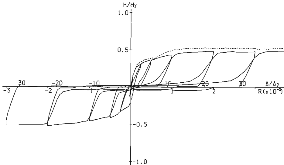
Fig. 10. H/H_y - \Delta/\Delta_y Relation of Round Bar Braces.
