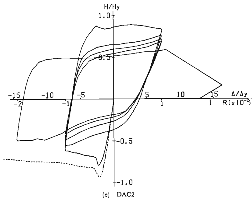
Fig. 8. H/H_y - \Delta_y Relation of Angle Braces.
