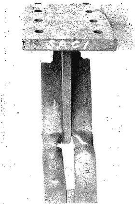
Photo. 13. Breakage due to Low Cycle Fatigue (SAC1).
