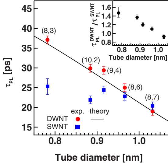
FIG. 4. (Color online) PL lifetimes \tau_{\text{PL}}^{\text{DWNT}} and \tau_{\text{PL}}^{\text{SWNT}} as a function of tube diameter in the DWNTs and SWNTs are denoted by solid circles and squares, respectively. The solid line shows the theoretically calculated curve using Eq. (3). The inset shows the PL lifetime ratio of DWNTs to SWNTs \tau_{\text{PL}}^{\text{DWNT}}/\tau_{\text{PL}}^{\text{SWNT}} as a function of the tube diameter.
