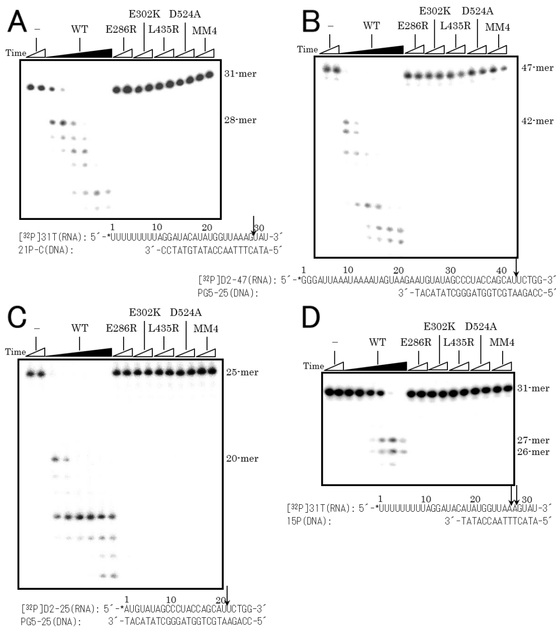
Fig. 5. RNase H activity. Reactions were carried out at 37°C for 0-40 min in the presence of 20 nM labelled T/P and 0 or 150 nM RT. The arrows indicate the cleavage sites. Labelled T/P: A, [ 32 P]31T(RNA)/21P-C(DNA); B, [ 32 P]D2-47(RNA)/PG5-25(DNA); C, [ 32 P]D2-25(RNA)/PG5-25(DNA); D, [ 32 P]31T(RNA)/15P(DNA). The asterisk indicates the position of the 32 P label. Time points were 0.25, 0.50, 2.0, 4.0, 20, and 40 min for WT and 0.25 and 40 min for mutant RTs.
