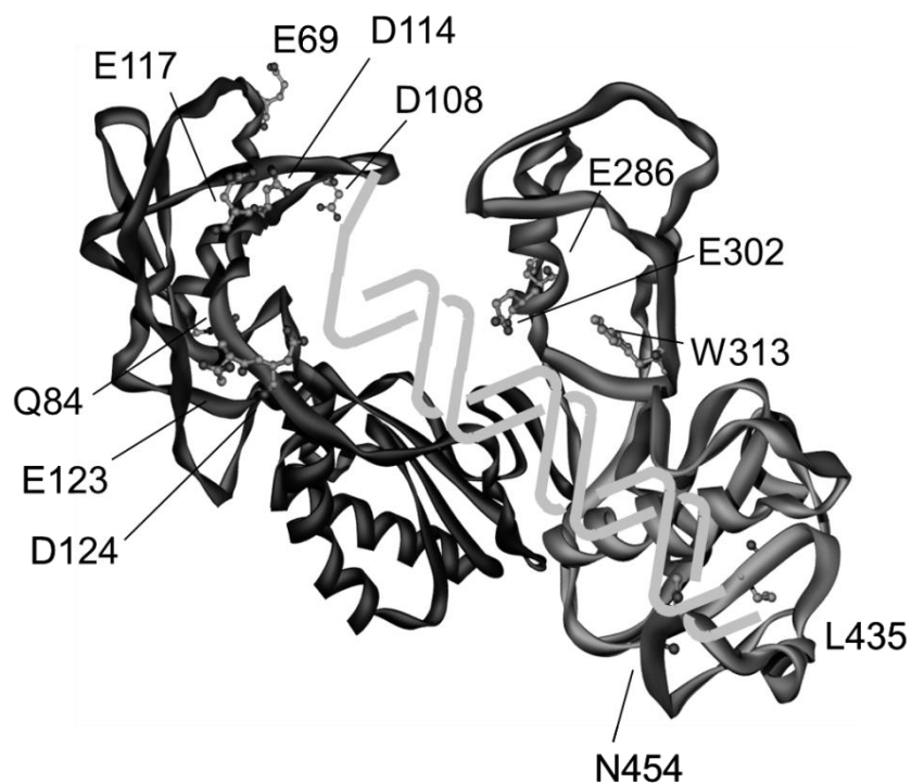
Fig. 1. Overall structure of MMLV RT. The structure is based on Protein Data Bank number 1RW3 (6). Peptide chain is displayed by a ribbon model. Residues subject to mutation are displayed by ball and stick. Template-primer (T/P) is schematically shown based on its presumed trajectory exiting the polymerase active site of MMLV RT (6).
