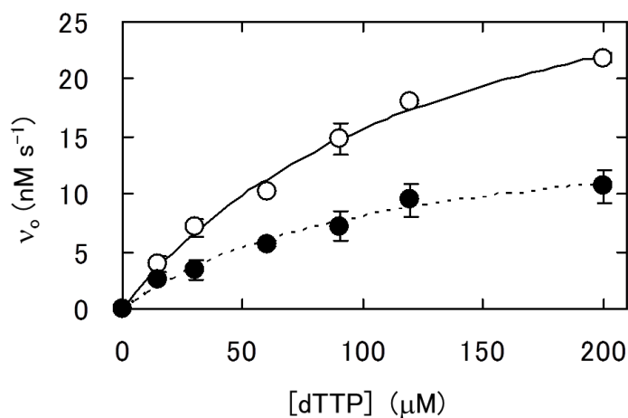
Fig. 3. Dependence on substrate concentration of the initial reaction rate of the RT-catalyzed reverse transcription reaction. The reaction was carried out with AMV RT \alpha\beta heterodimer (open circle) and \alpha subunit (closed circle) at 10 nM at 37°C. The concentration of poly(rA)-p(dT) 15 was 25 \mu M. Error bars indicate SD values for triplicate measurements. Solid and broken lines represent the best fit of the Michaelis-Menten equation by the non-linear least squares method.
