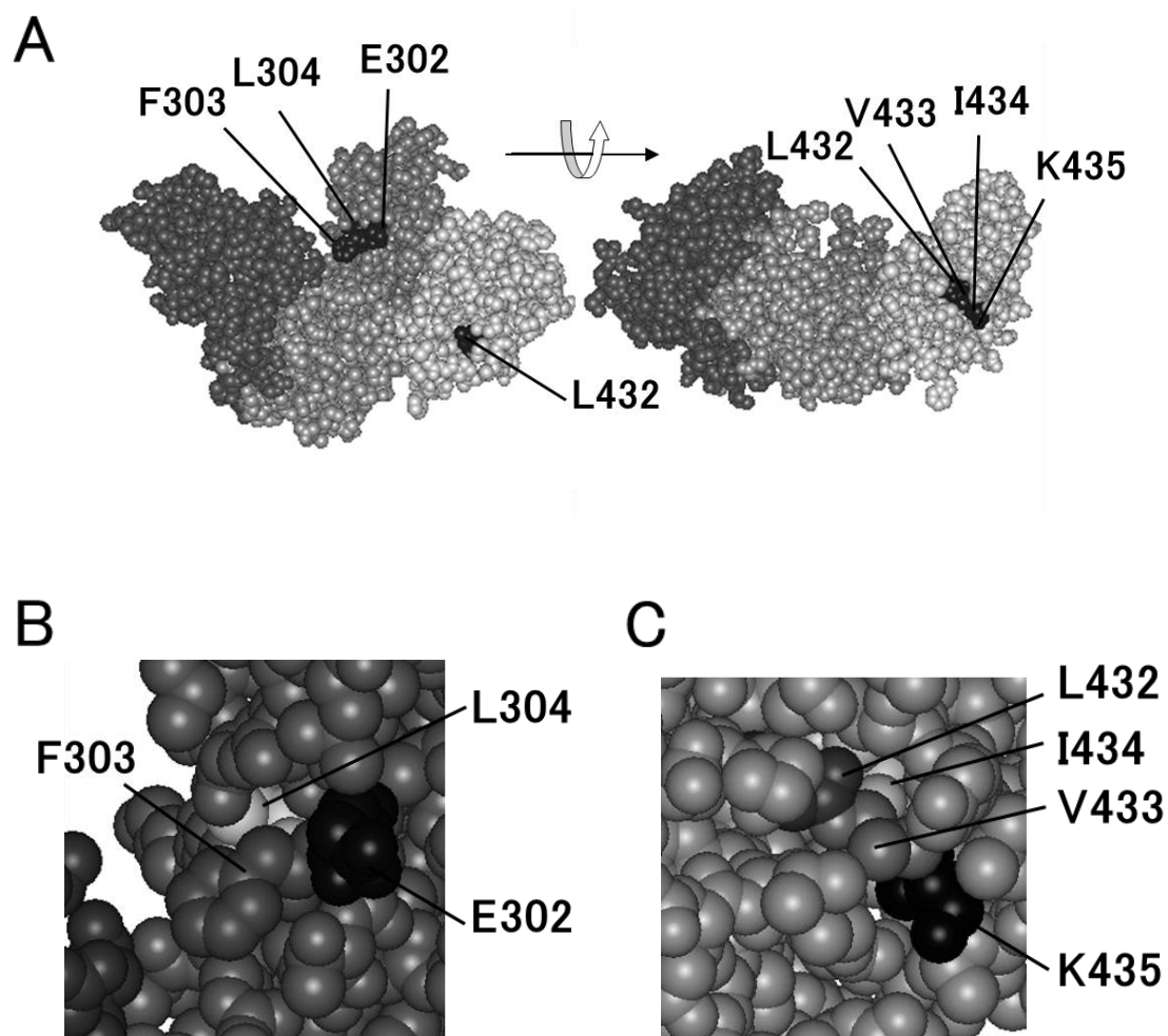
Fig. 6. Structure of MMLV RT variant L435K. The structure is based on Protein Data Bank no. 1RW3. (A) Overall structure. (B) Close-up view of the surface region, in which Phe303 and Leu304 are located. (C) Close-up view of the surface region, in which Leu432, Val433, and Ile434 are located.
