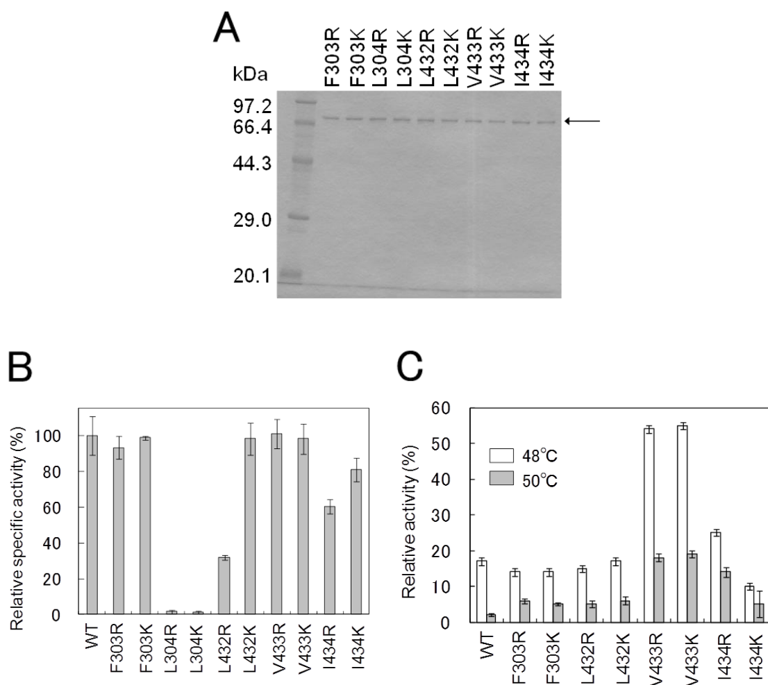
Fig. 7. Analysis of single MMLV RT variants. (A) SDS-PAGE under reducing conditions. Coomassie Brilliant Blue-stained 10% SDS-polyacrlamide gels is shown. The arrow indicates the band corresponding to MMLV RT. (B) Specific activity. One unit was defined as the amount that incorporates 1 nmol of dTTP into poly(rA)-p(dT) 15 in 10 min. Relative specific activity was defined as the ratio of the specific activity of RT to that of WT (34,000 units/mg). (C) Thermal stability. RT at 50 nM was incubated at 48 or 50°C for 10 min. Then a dTTP incorporation reaction was carried out at 37°C. Relative activity was defined as the ratio of the initial reaction rate of RT with 10 min incubation at 48 or 50°C to that without the incubation.
