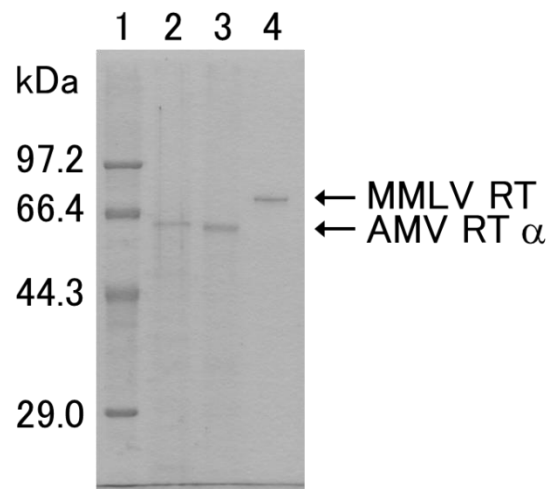
Fig. 5. SDS-PAGE under reducing conditions. Coomassie Brilliant Blue-stained 10% SDS-polyacrylamide gel is shown. Lane 1, molecular-mass marker; lane 2, wild-type AMV \alpha subunit (WT); lane 3, AMV RT \alpha subunit variant V238R/L388R/D450A (AM4); lane 4, wild-type MMLV RT.
