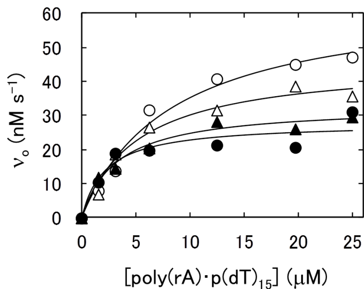
Fig. 3. Dependence on substrate concentration of the initial reaction rate of RT-catalyzed incorporation of dTTP into poly(rA)-p(dT) 15 at 37°C. The initial concentrations of RT and dTTP were 5 nM and 200 μM, respectively. Solid lines represent the best fit of the Michaelis-Menten equation with the non-linear least squares method. Symbols for the enzymes: WT, open circle; D524A, open triangle; MM3, closed circle; MM4, closed triangle.
