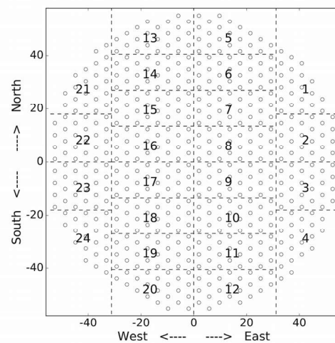
Figure 1. EAR antenna array
