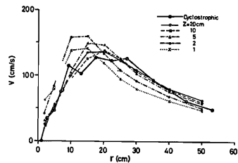
Fig. 12 Comparison of the cyclostrophic wind with the measured tangential winds for Case III.
