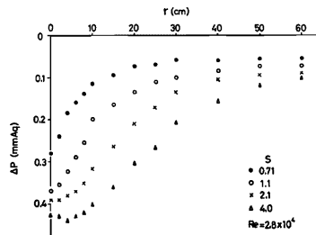
Fig. 11 Radial distribution of the surface pressure.
