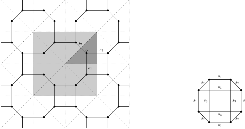
FIGURE 4. The Cayley graph of the affine Weyl group (\Gamma, S) of type \tilde{C}_2 and the action on \mathbb{R}^2 (left), and the quotient graph G = \mathbb{Z}^2 \backslash \text{Cay}(\Gamma, S) (right).
