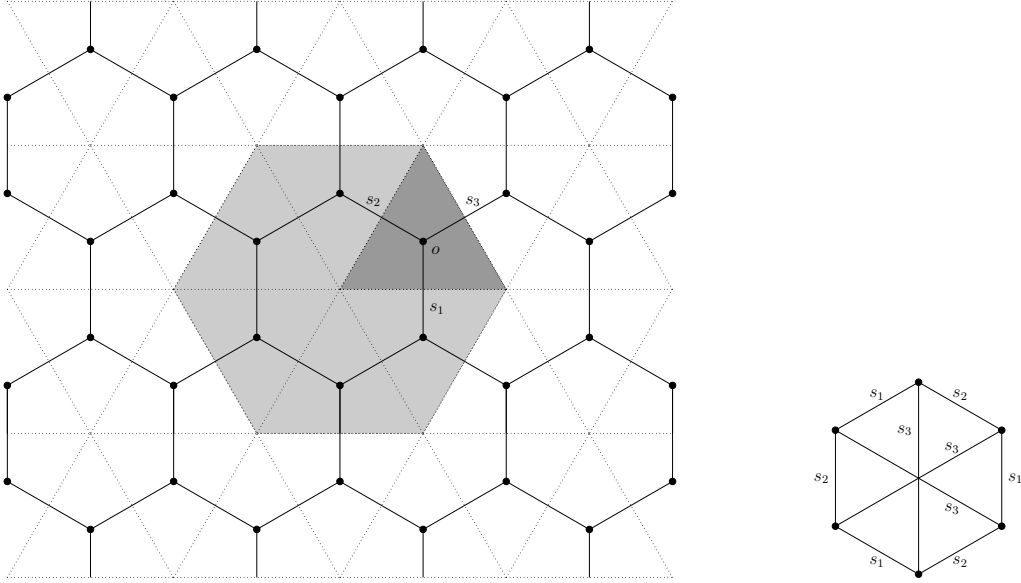
FIGURE 3. The Cayley graph of the affine Weyl group (\Gamma, S) of type \tilde{A}_2 and the action on \mathbb{R}^2 (left), and the quotient graph G = \mathbb{Z}^2 \backslash \text{Cay}(\Gamma, S) (right).
