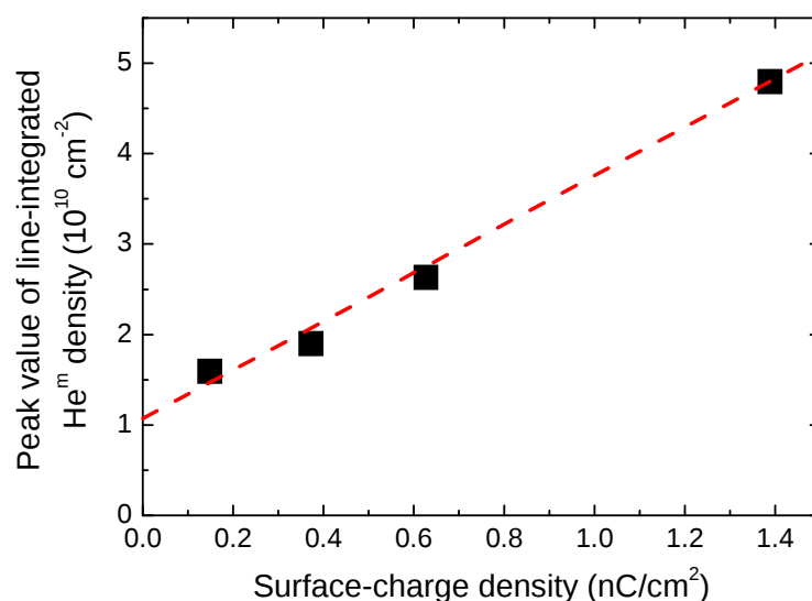
Figure 3.13 Relationship between surface-charge density accumulated owing to coaxial DBD inside tube and peak line-integrated \text{He}^{\text{m}} density in plasma plume, measured 10 mm from tube exit. Red dotted line shows linear fit of these four experimental results.
