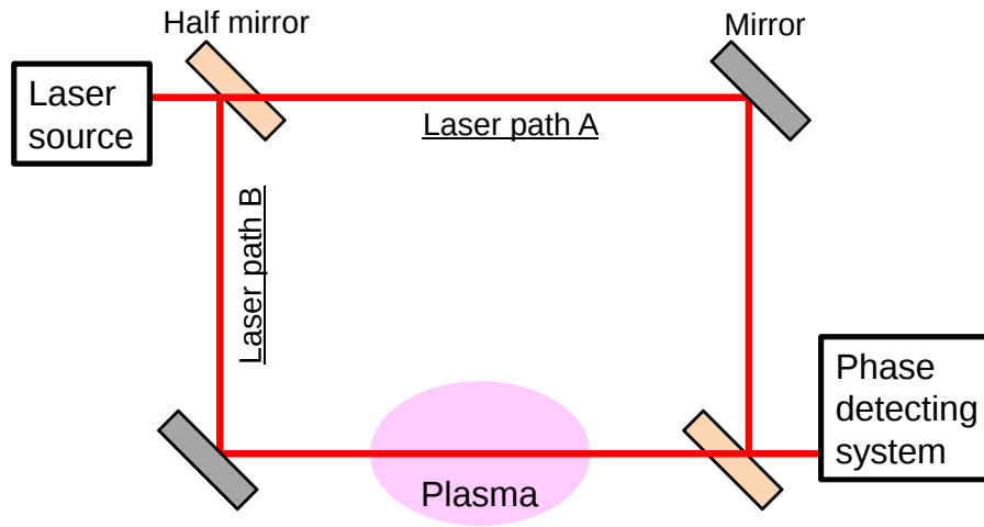
Figure 1.5 Schematic diagram of laser interferometry using Mach-Zehnder configuration for electron-density measurement inside plasma source.
