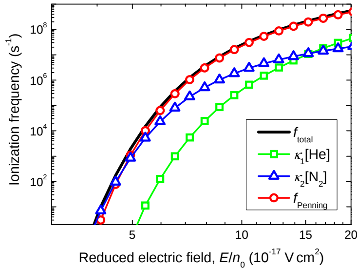
Figure 2.15 Calculation results of total ionization frequency f_{\text{total}} and ionization frequencies associated with electron impact ionizations of He atoms ( \kappa_1[\text{He}] ) and N_2 molecules ( \kappa_2[\text{N}_2] ) and two- and three-body Penning ionizations between He^m atoms and N_2 molecules ( f_{\text{Penning}} ) as a function of reduced electric field E/n_0 in 0.25% condition of N_2 impurity ratio.
