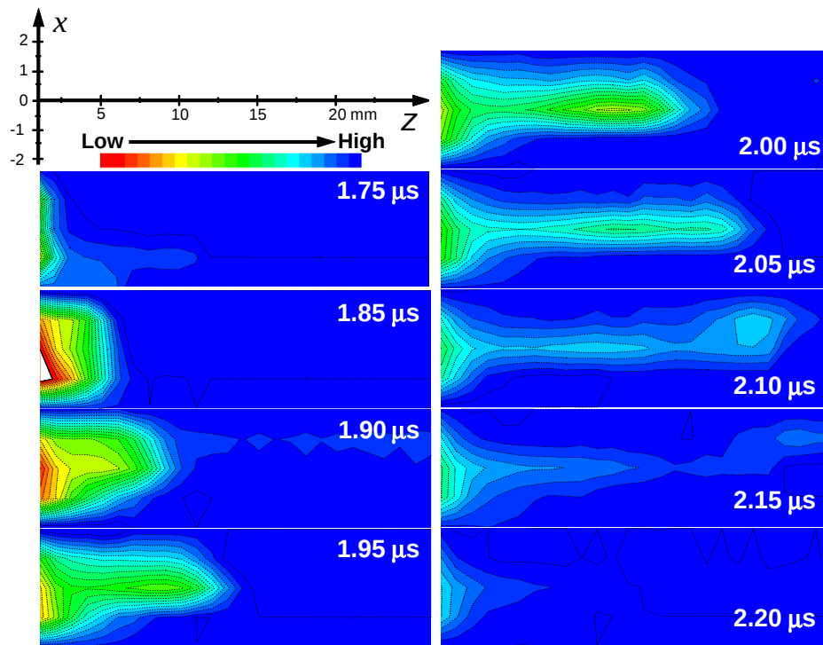
Figure 4.4 Spatiotemporal distributions of line-integrated He m absorption in contour diagram (with color code) in the positive voltage phase without grounded plate with V_{0p} = 6.0 kV and d_{\text{tube}} = 4 mm (white region indicates the overflowed region with absorption more than 0.024). Time scale is matched with abscissa axis of Fig. 4.2.
