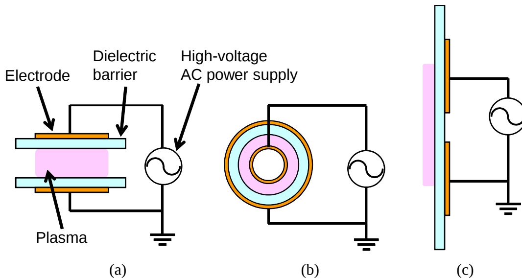
Figure 1.10 Two-dimensional schematic diagrams of electrode structures used for dielectric barrier discharge, (a) parallel plate type, (b) tubular type, and (c) surface barrier discharge type.
