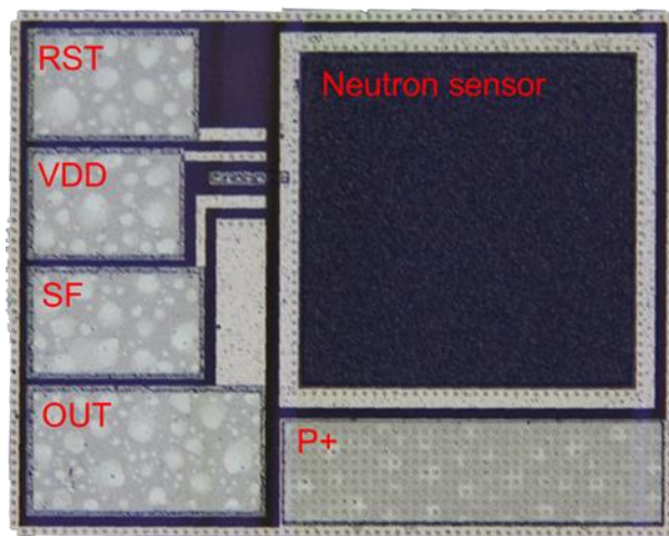
Fig. 1. SiC Neutron Sensor: This sensor consists of neutron sensor and three transistors.
