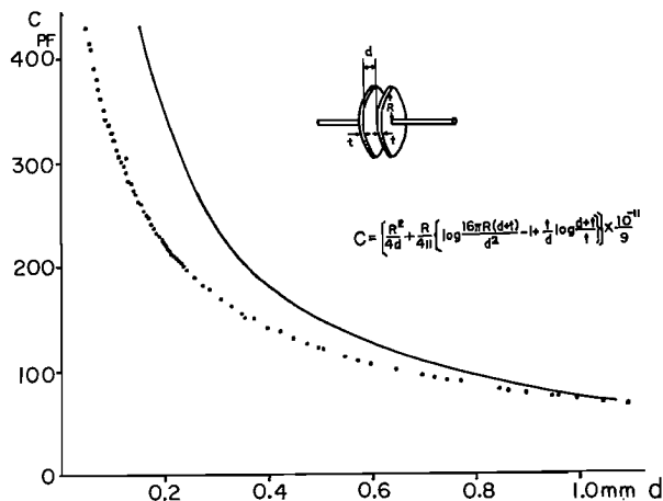
Fig. 2. Change of the capacitance versus the distance between the plates.
