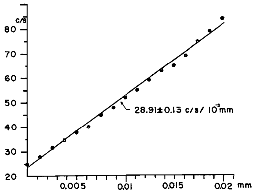
Fig. 10. Frequency change versus the distance between the plates when multiplied up to 10 Mc/s.
