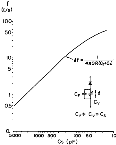
Fig. 3. Frequency change to the capacitance C_s .
