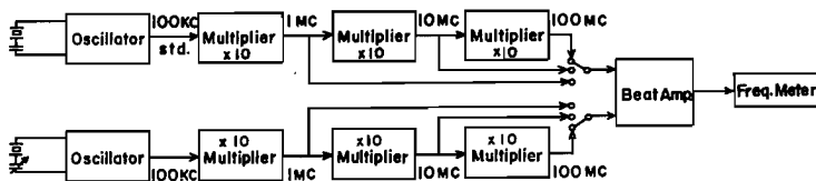
Fig. 1. Block diagram of the extensometer.
