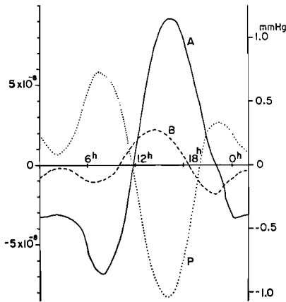
Fig. 9. Mean daily variations of the ground strains observed by the extensometers of the variable capacitor type (A) and of the bow-string type (B) and the atmospheric pressure (P).
