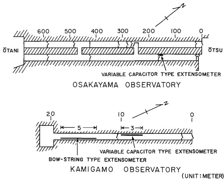
Fig. 6. Plane figures of the observatories and locations of the instruments.
