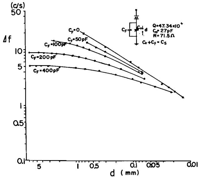
Fig. 4. Frequency changes versus the distance between the plates.
