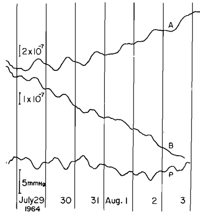
Fig. 8. Comparison among the ground strains observed by the extensometers of the variable capacitor type (A) and of the bow-string type (B), and the atmospheric pressure (P).
