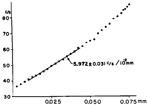
Fig. 7. Frequency change versus the distance between the plates when multiplied up to 10 Mc/s.
