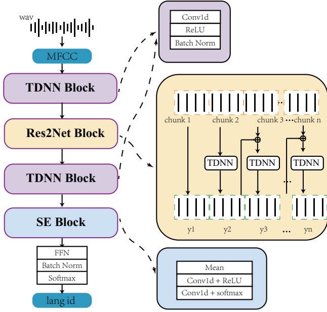
Fig. 2. Illustration of the SLI model architecture.
