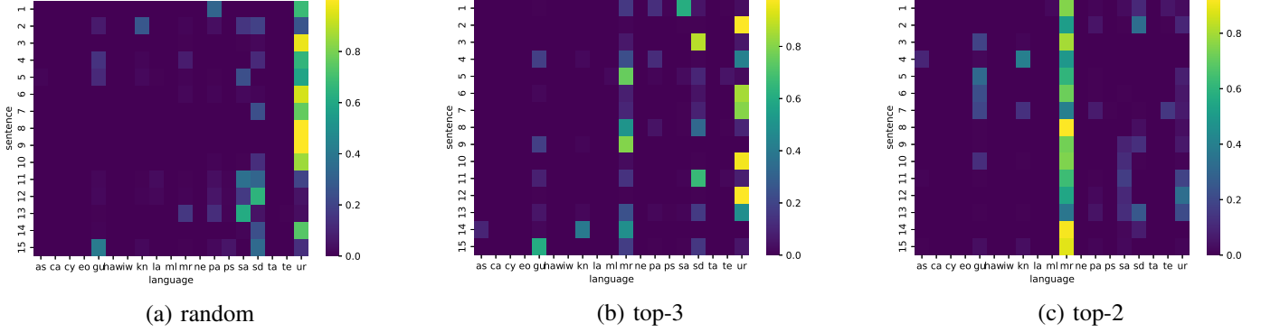
Fig. 3. Probabilities of the Hindi data with different data selection methods on 19 languages (as, ca, cy, eo, gu, haw, iw, kn, la, ml, mr, ne, pa, ps, sa, sd, ta, te, ur). (a) is the probabilities for random selection; (b) is for SLI selection with k=3 ; (c) is with k=2 .
