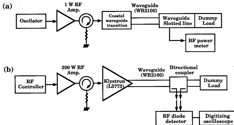
Figure 5. Schematic block diagram of the low power (a) and the high power measurement setup (b) of the return loss of the dummy-load.
