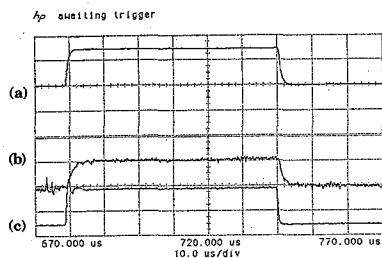
Figure 7. The RF pulse shapes of the input and output power of the dummy-load. The RF frequency is 433.3 MHz. Time base is 10 \mu sec/div.
