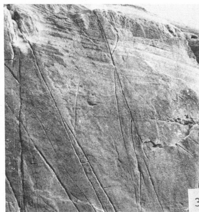
Plate II Sedimentary features of thick-bedded sandstones
