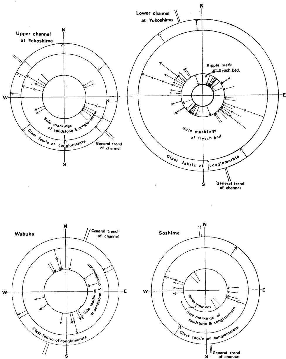
Fig. 24. General trends of channels and paleocurrents in each channel-filling sediments.
