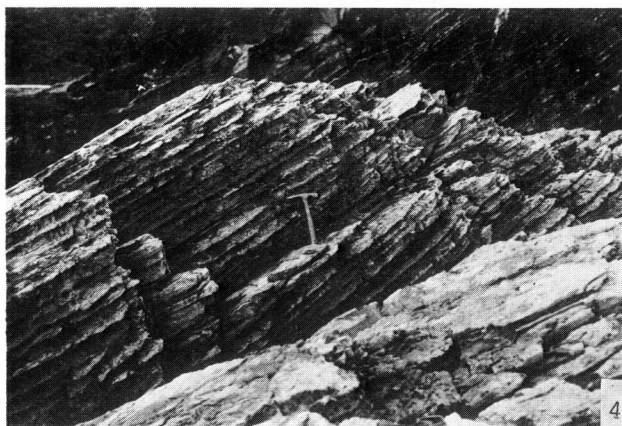
Plate IV Flysch-type alternation
