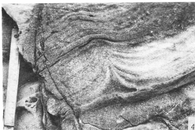
Plate III Internal sedimentary structures of thick-bedded sandstones
